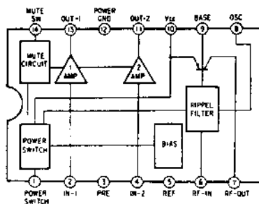
IC304 LA4538M
