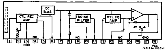
BX3914 (SONY) CTL REC/P8 AMPLIFIER - PRINTED SIDE -
