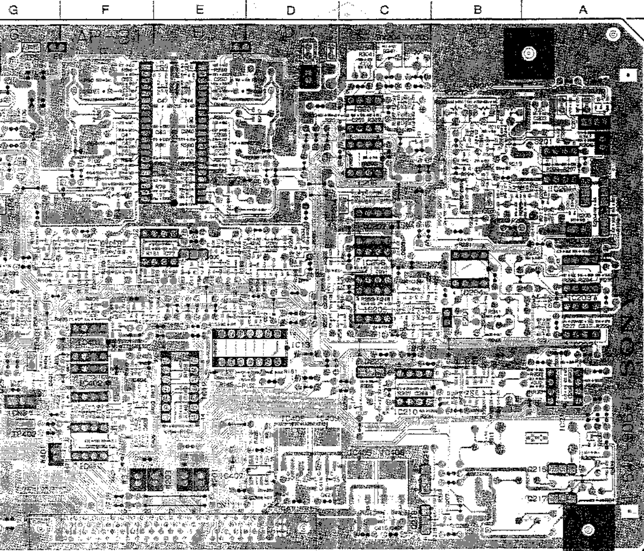
AP-31 1-648-906-11 B SIDE
