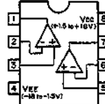
TL062CPS (TI) FLAT PACKAGE TL062CPS (TI) FLAT PACKAGE OPERATIONAL AMPLIFIER (JFET INPUT) - TOP VIEW -
