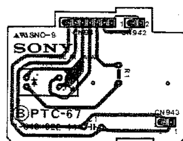
PTC-67 1-648-922-11 B SIDE
