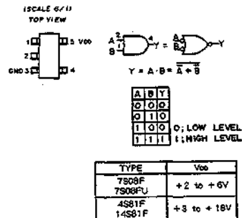
TC7308F (TOSHIBA) CHIP PACKAGE CMOS 2-INPUT AND GATE
