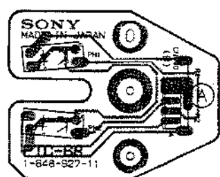
PTC-68 1-648-927-11 A SIDE
