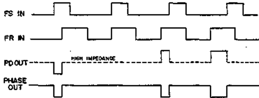
PHASE COMPARATOR TIMING CHART
