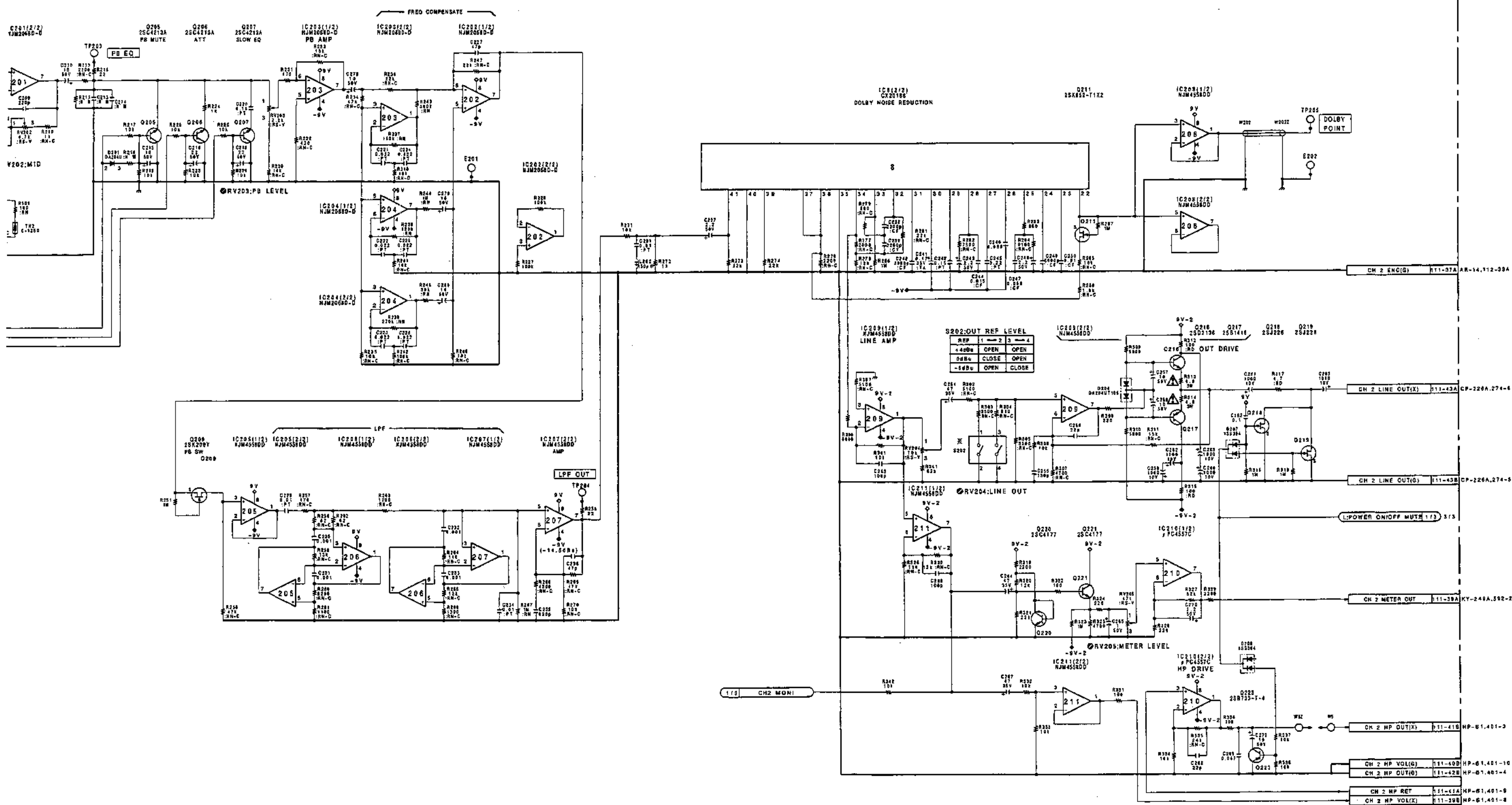
AP-31A BOARD ( 2 / 3 )
