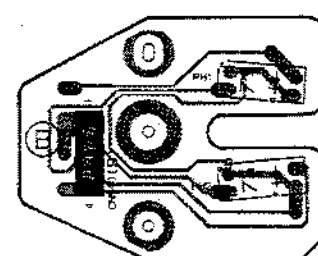
PTC-68 1-648-927-11 B SIDE
