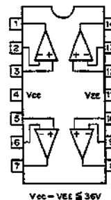
UPC4574G2 (NEC) QUAD OPERATIONAL AMPLIFIER - TOP VIEW -
