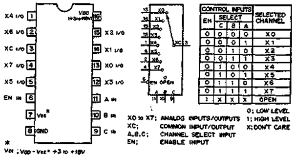
MC14052BF (MOTOROLA) FLAT PACKAGE CMOS DUAL 4-CHANNEL ANALOG MULTIPLEXERS/DEMULTIPLEXERS - TOP VIEW -
