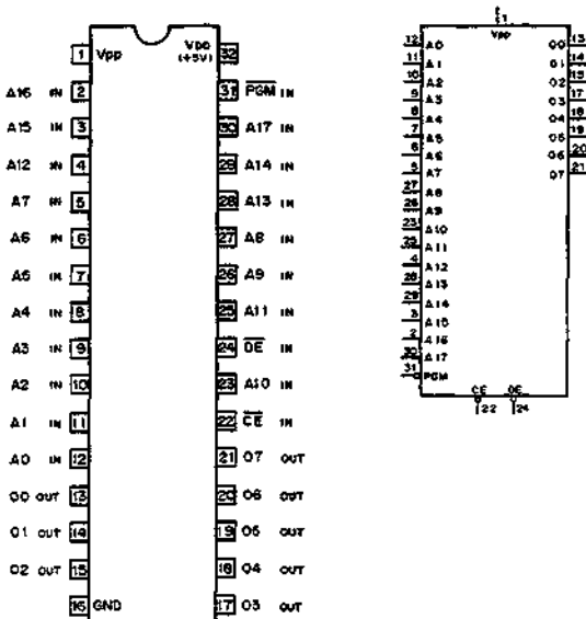
AM27C020-150DC (AMD) C-MOS 2M (256,144x8)-BIT UV ERASABLE PROM - TOP VIEW -
