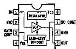
CXA1521M (SONY) GAIN CONTROL AMP - TOP VIEW -
