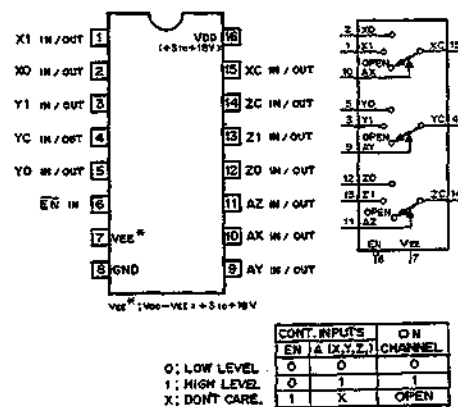
MC14053BCP (MOTOROLA) MC14053BF (MOTOROLA) FLAT PACKAGE UPD4053BC (NEC) CMOS TRIPLE 2-CHANNEL ANALOG MULTIPLEXERS/DEMULTIPLEXERS - TOP VIEW -
