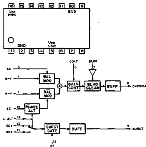
CX22017 (SONY) VIDEO SIGNAL PROCESSOR - TOP VIEW -
