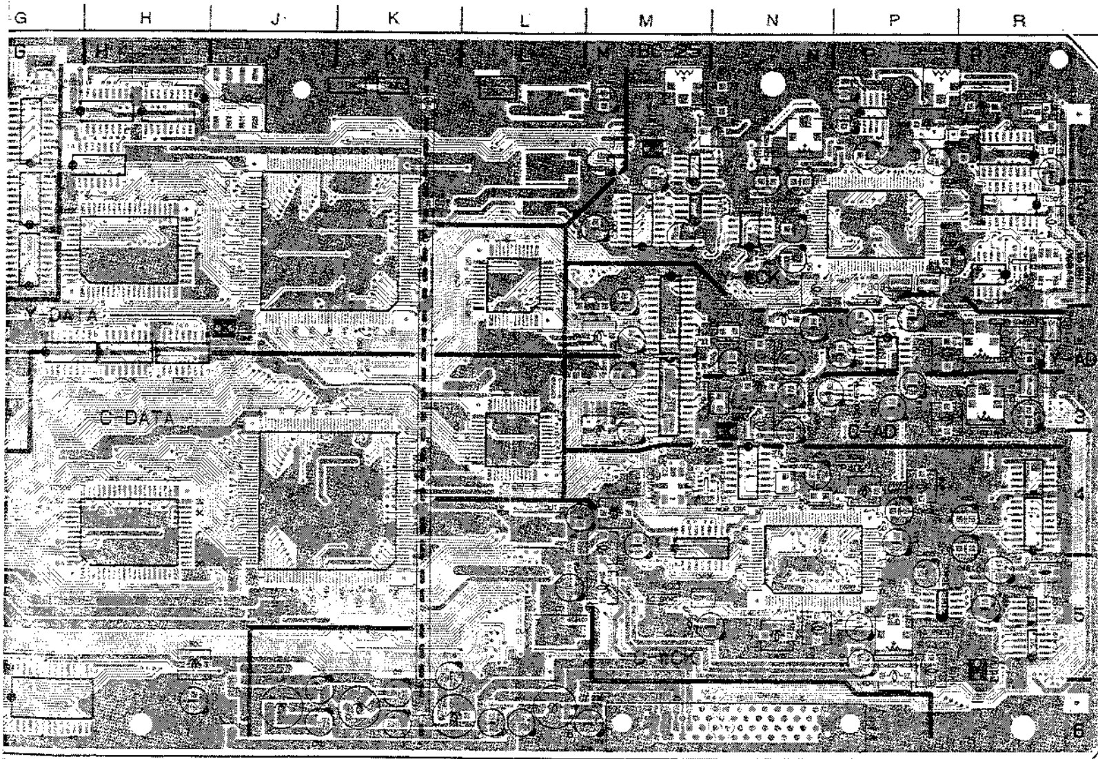
TBC-25 1-648-901-11 A SIDE
