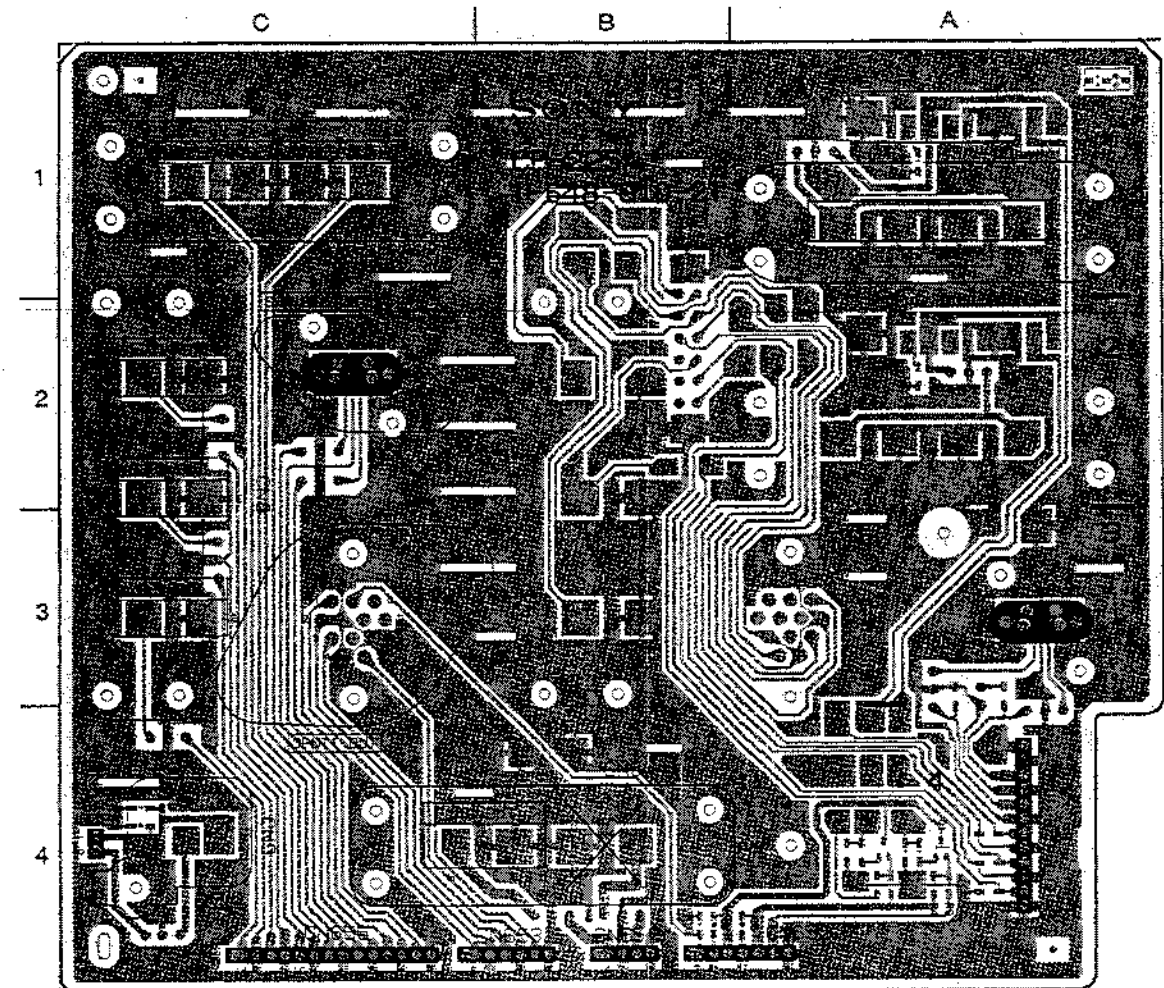
CP-225A 1-648-910-21 B SIDE
