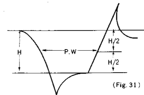
Waveform of Transistor X_{501} Emitter
