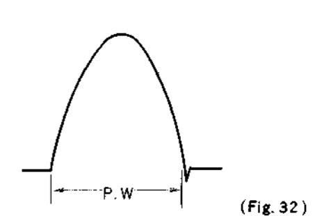
Waveform of Transistor X_{502} Collector
