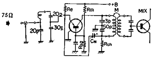
For 5-303E (Fig. 17-1)
