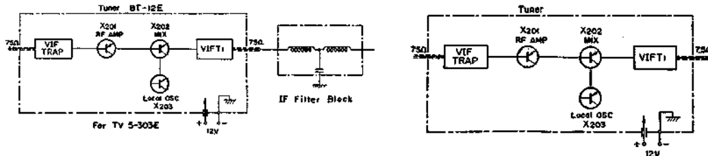
For 5-303E (Fig. 14-1)
