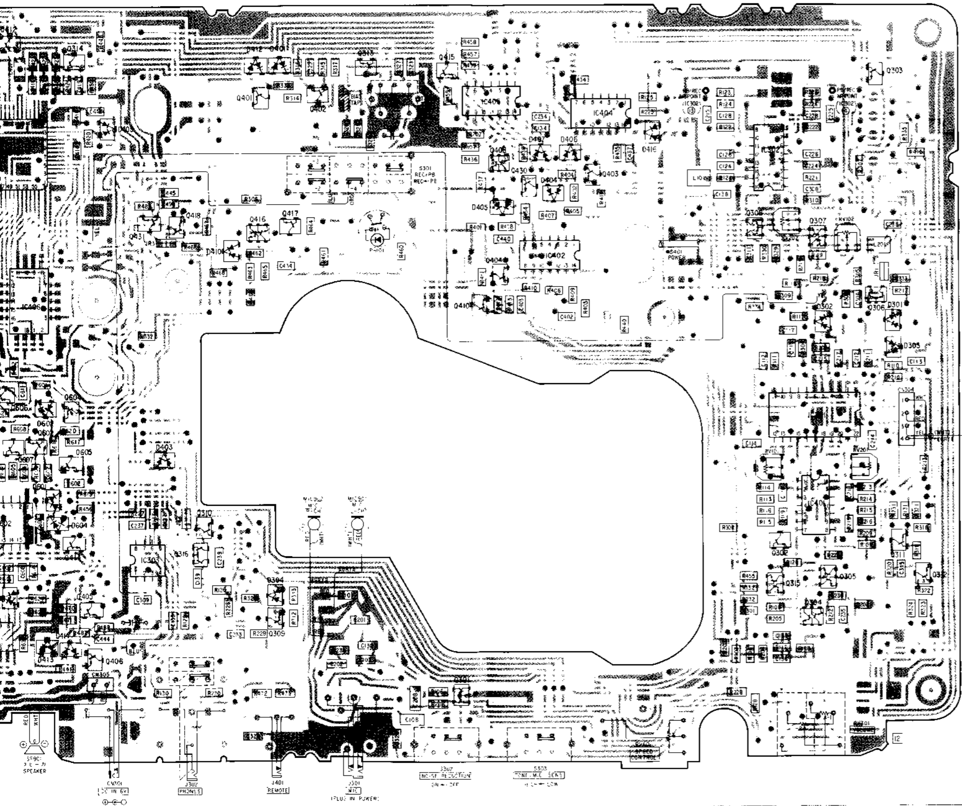
[SWITCH FLEXIBLE BOARD] [スイッチフレキ基板]
