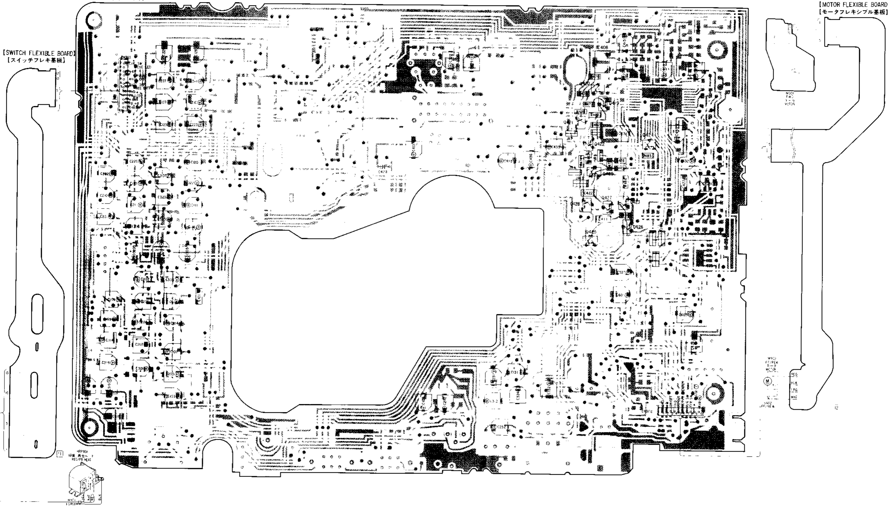
[MAIN BOARD (B SIDE)] [メイン基板(B面側)]
