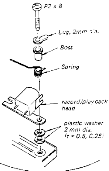
record/playback head
