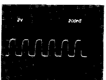
⑦② IC508⑦② 4.0Vp-p
