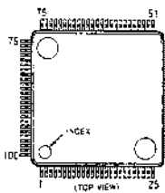
CXK58257ATM-12LB
