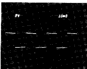
⑦② IC506⑦② } 4.0Vp-p ⑬② IC508⑬② } TP (DREF)
