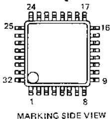
MM1138XQ
