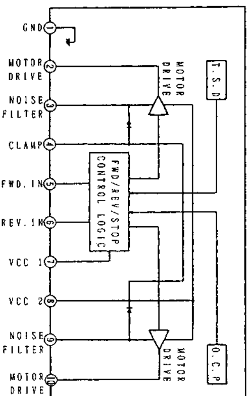
● IC Block Diagram IC805, 807 BA6219B IC803, 806, 808 LB1641
