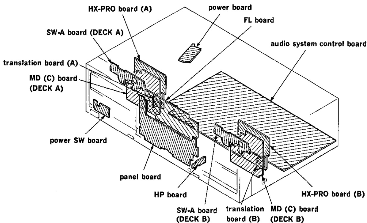
5-1. CIRCUIT BOARDS LOCATION (TC-WR720A)
