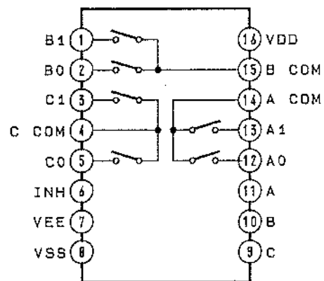
μPD4053BC
