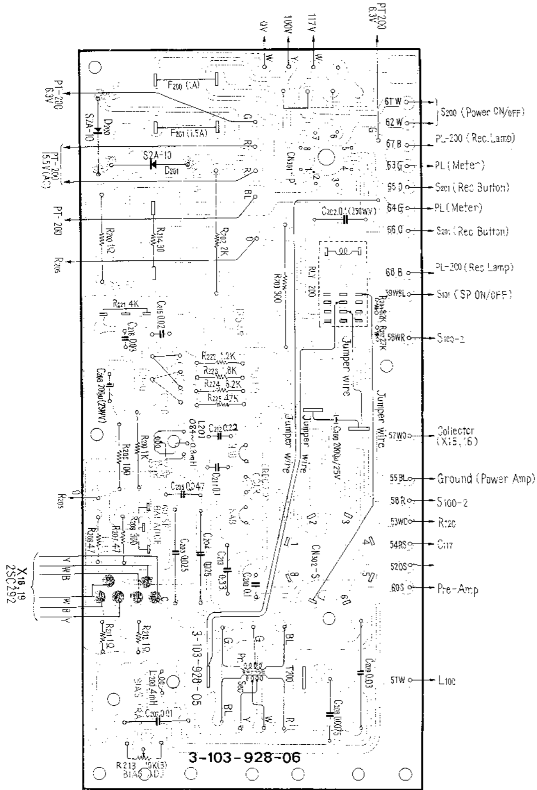
Power Supply & Bias OSC Section Conductor Side -
