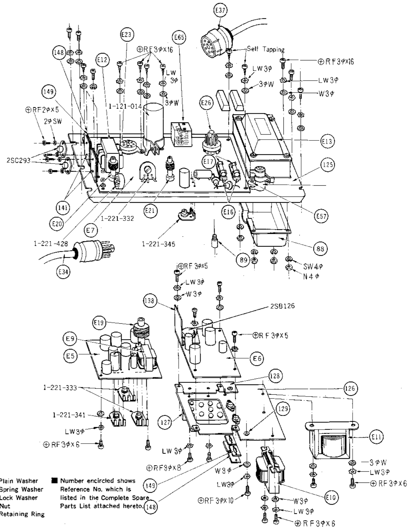
Amplifier Chassis—Top View
