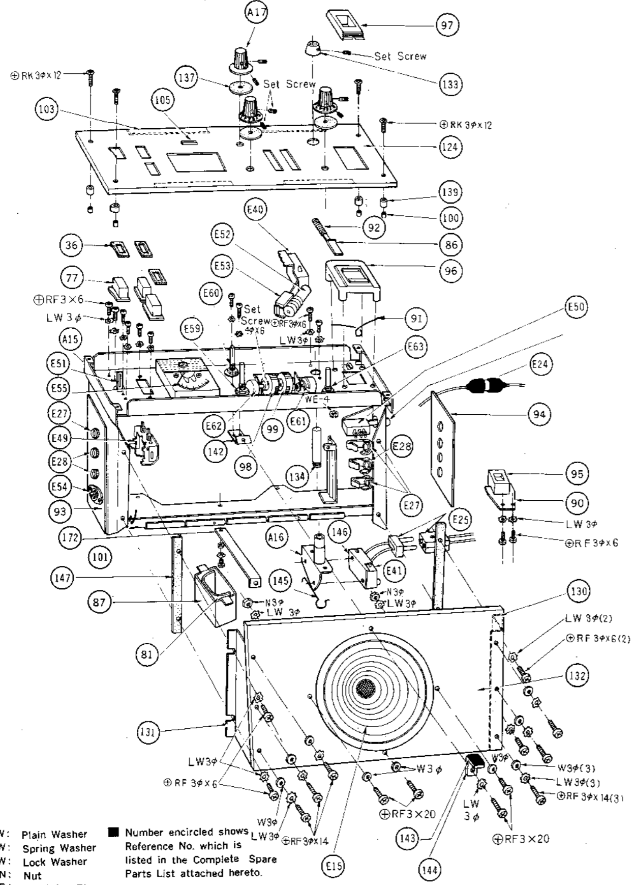
Front Chassis—Top View
