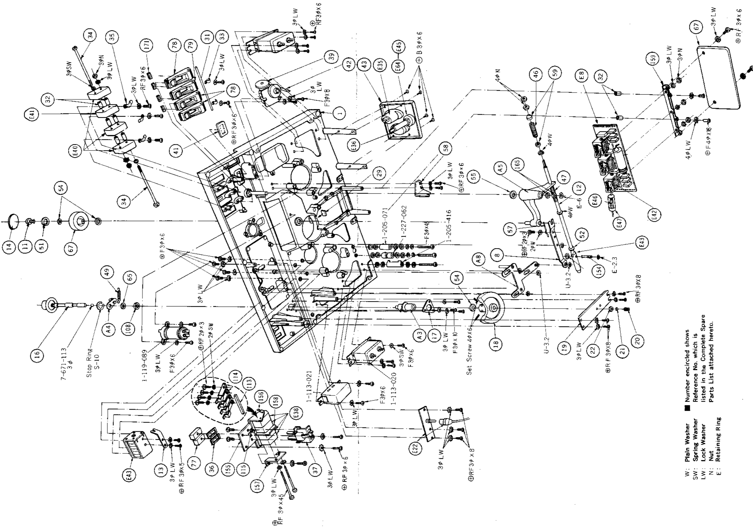
Exploded Diagram Chassis—Bottom View
