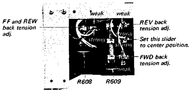
Fig. 3-13. Back tension torque adjusting parts location
