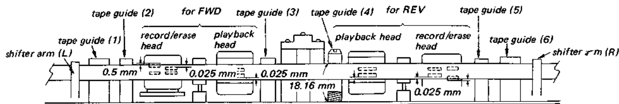
Fig. 3-26. Head adjustment
