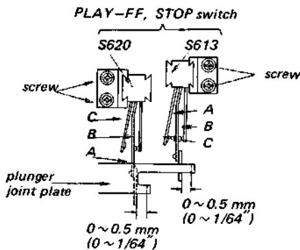
Fig. 3-22. PLAY-FF, STOP switch (S613, 620) position adjustment
