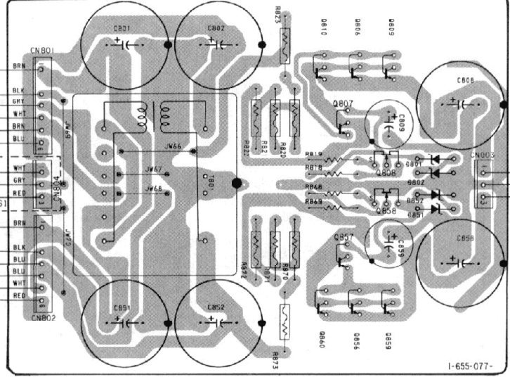
[PRE PS BOARD]
