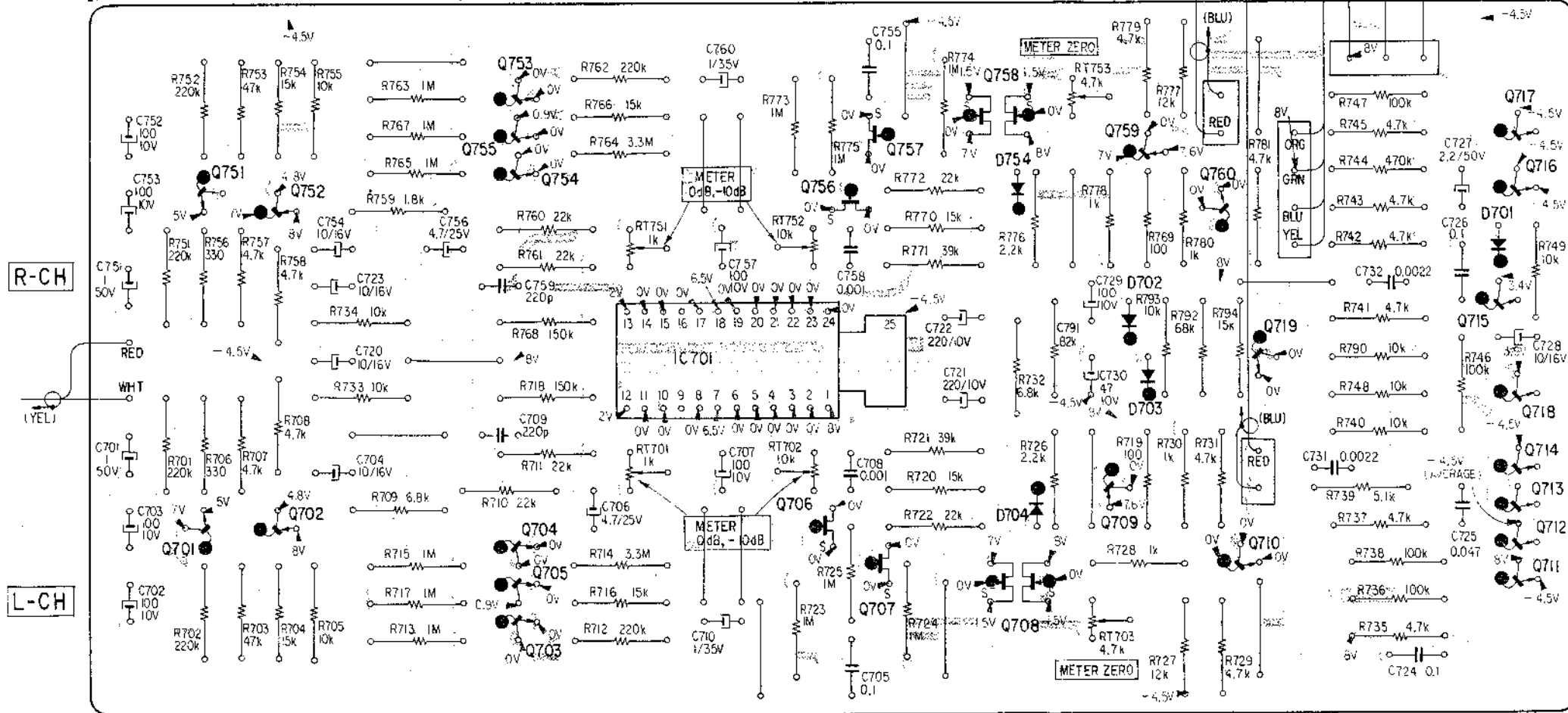
[METER AMP BOARD] (CONDUCTOR SIDE)
