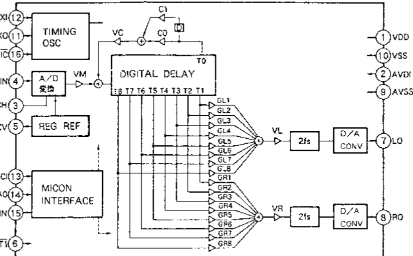
IC301 YM7128
