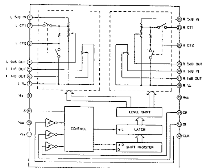
IC550, 555 LC7535
