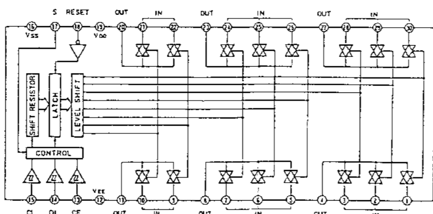
IC104, 105, 701, 702 LC7822
