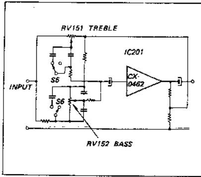
Fig. 1-2. Simplified tone control circuit
