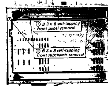
Fig. 2-1. Front panel and front subchassis removal
