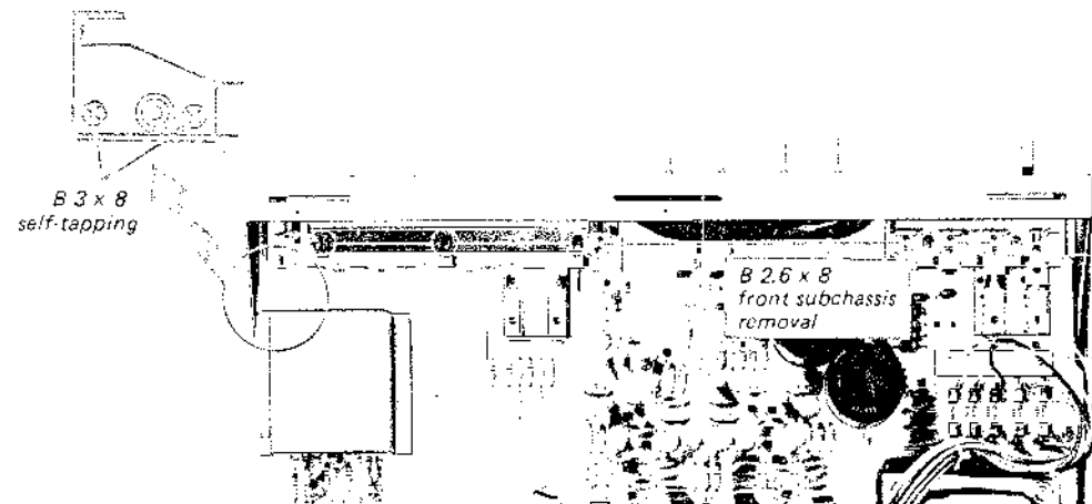
Fig. 2-3. Front subchassis removal
