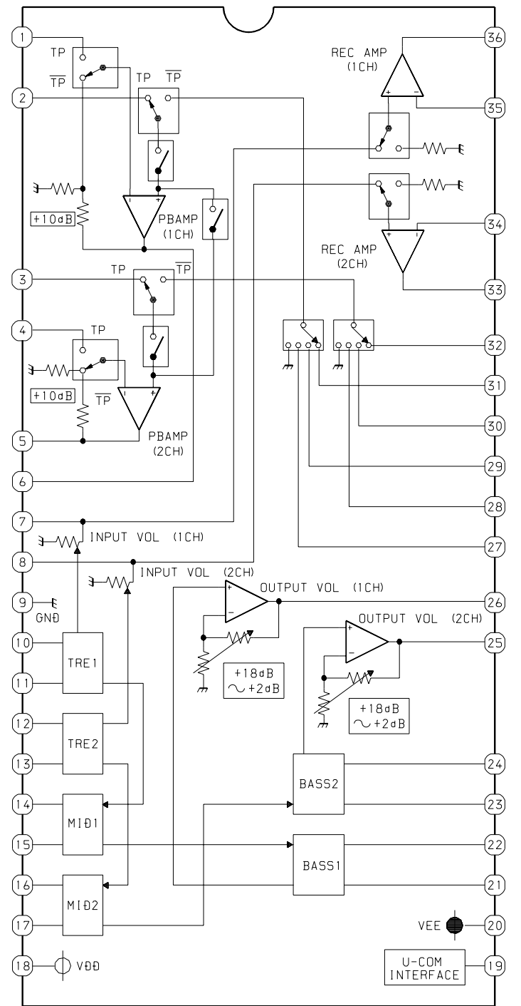
IC, M61518FP
