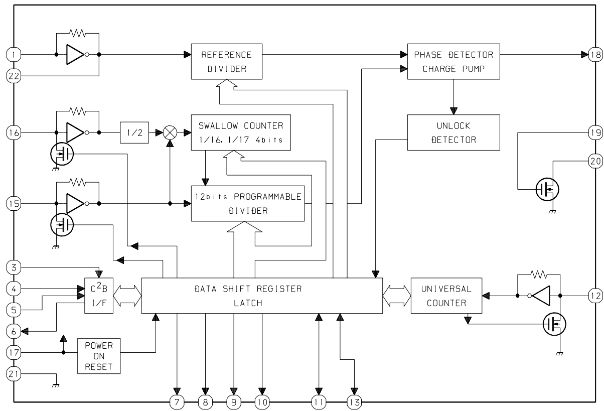
IC, LC72131D-N
