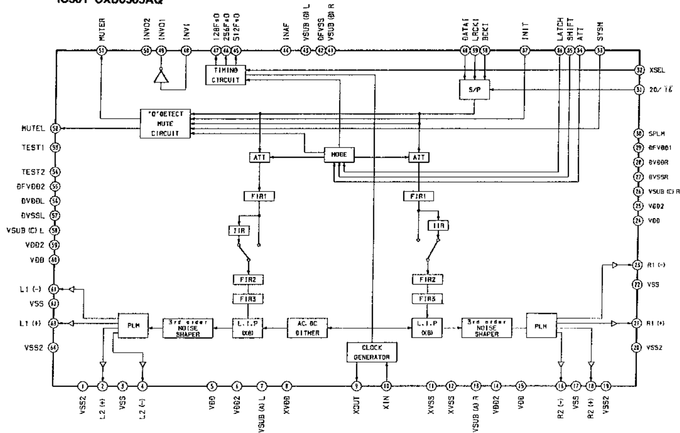
IC501 CXD8505AQ
