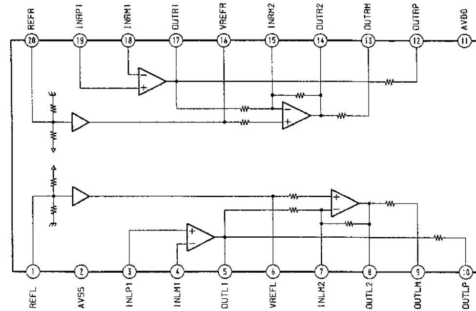
IC505 CXA8043M
