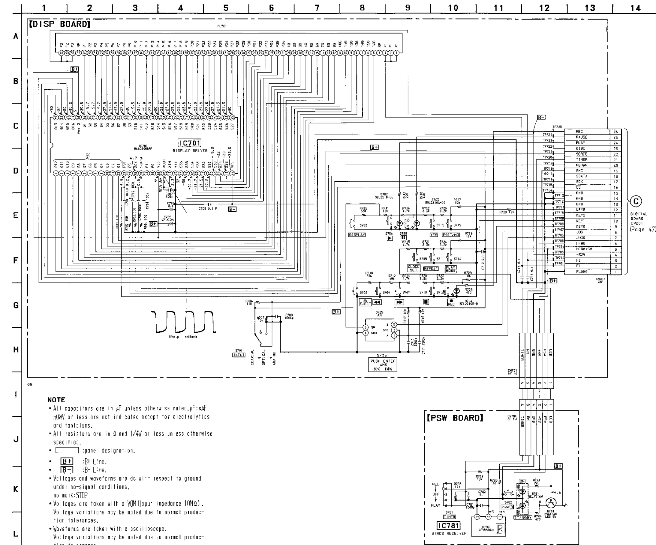
5-10. SCHEMATIC DIAGRAM — PANEL SECTION —
