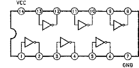
IC906 SN74HC04N
