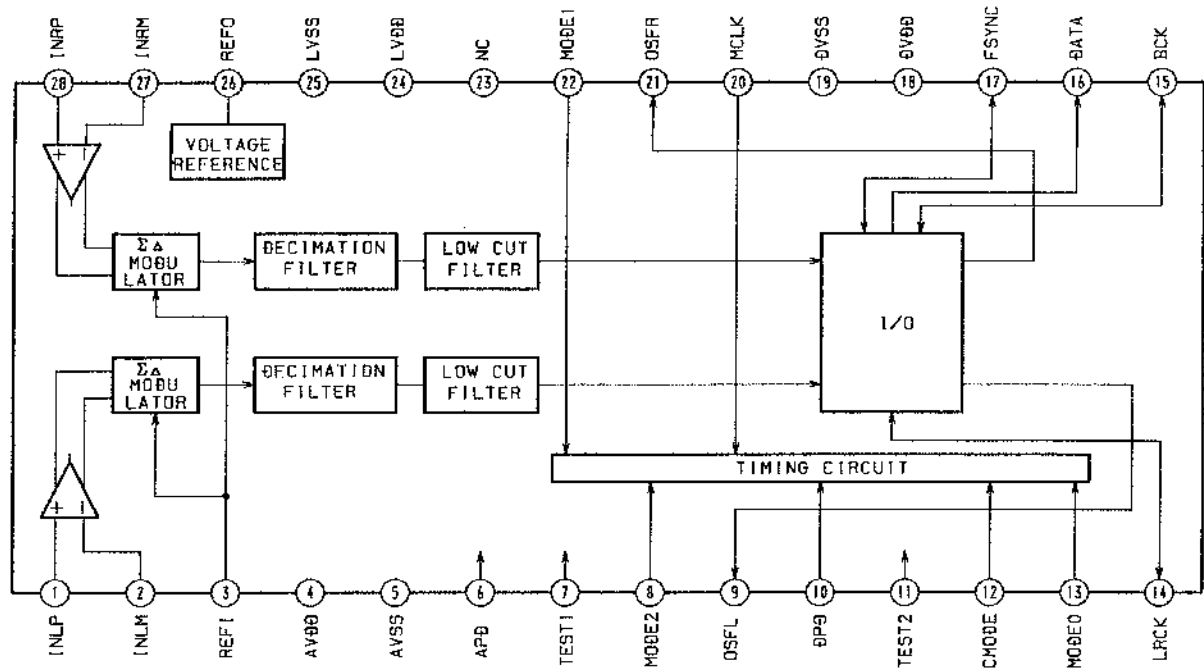
IC502 CXD8539M
