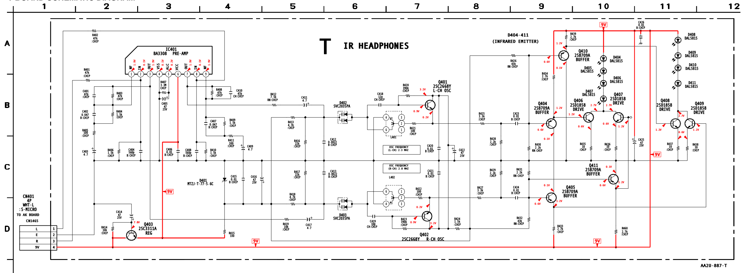
T BOARD SCHEMATIC DIAGRAM
