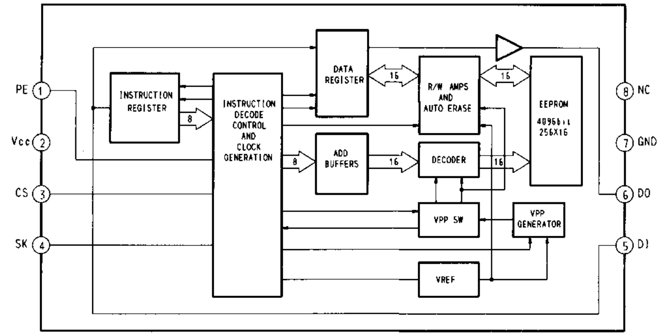
IC606 AK93C65LF-E1
