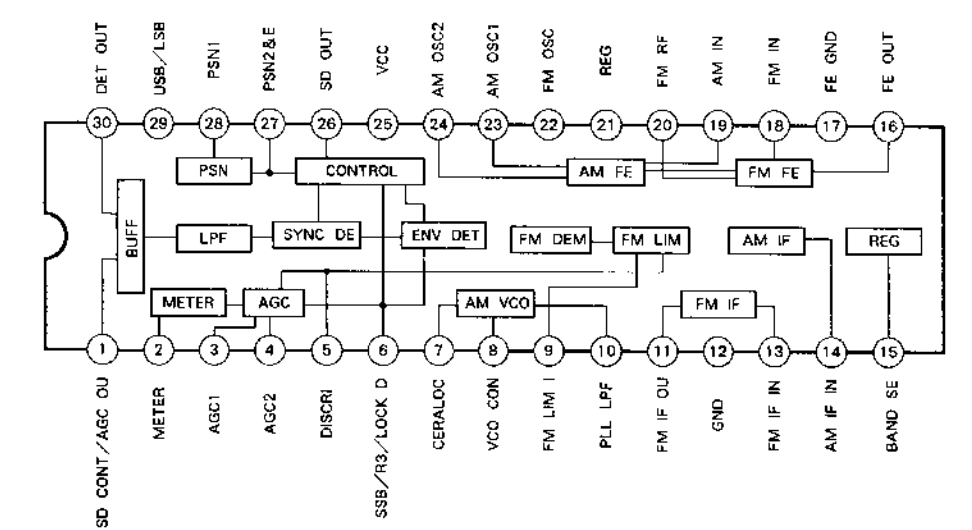
IC201 CXA1376AM
