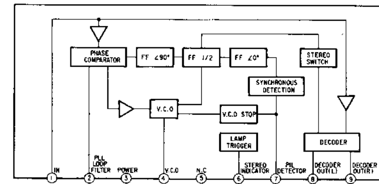
IC302 CXA1622M
