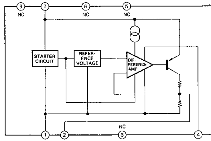
IC101 LA5002M
