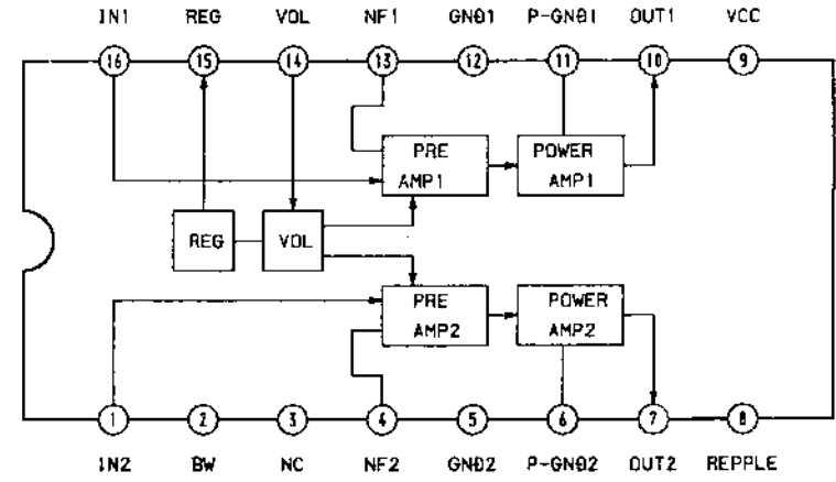
IC302 CXA1622M
