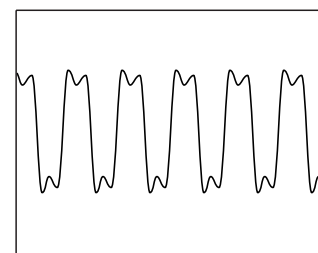
3.5 Vp-p (27 MHz)
