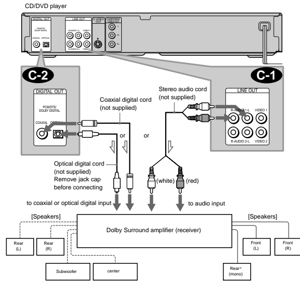
Signal flow *When connecting 6 speakers, replace the monaural rear speaker with a center speaker, 2 rear speakers and a subwoofer.
