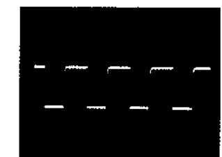
14 IC01 3pin, IC311 10pin (DFG) PLAY mode 5Vp-p, 1.25ms
