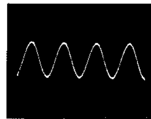
㉓ IC307 ⑬pin, (XT1I) 5.6Vp-p, 50ns
