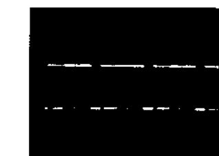
17 IC307 16pin, IC306 16pin (ADDT) REC mode 5.2Vp-p, 5μs
