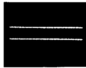
③ IC307 ⑦pin, IC311 ②pin (RFDT) PLAY mode 1Vp-p, 10ms
