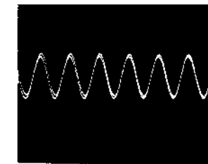
⑦ IC330 ⑩pin (XIN) 1.2Vp-p, 20μs
