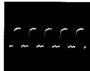
⑰ IC307 ②pin, IC311 ⑤pin, IC312 ③pin (MCLK) 5.8Vp-p, 50ns
