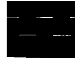
⑭ IC330 ⑩pin (XINTR) 5.2Vp-p, 0.1μs
