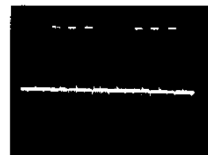
9 IC701 17-18pin, 1-18pin (a-v) 38Vp-p, 1.2ms
