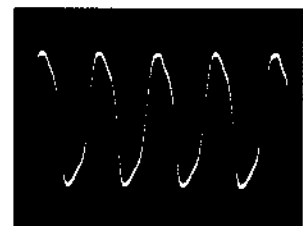
4 IC701 20pin (XTAL) 5.5Vp-p, 2.5μs
