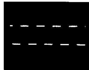
⑯ IC307 ④pin (PLCO) 4.8Vp-p, 0.18ms
