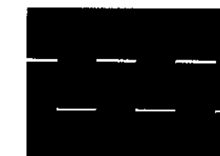
20 IC307 12pin (LRCK) 5.6Vp-p, 5μs
