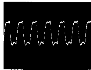
㉑ IC307 ⑤pin, IC359 ②pin (F256) 6.1Vp-p, 50ns
