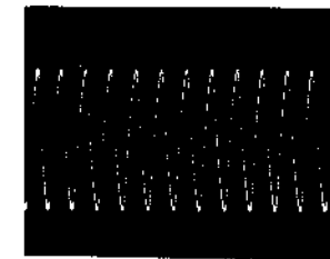
⑤ IC601 ⑩pin, IC363 ⑦pin (512FS) 4.5Vp-p, 50ns
