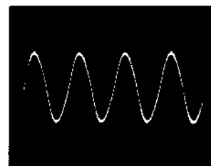
㉙ IC307 ⑬pin, (XT1O) 4Vp-p, 50ns
