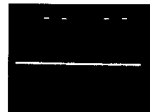
2 IC701 19-20pin (10G-1G) 34Vp-p, 2.45ms
