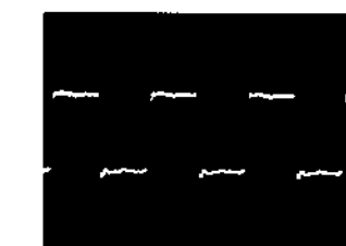
19 IC307 14pin, IC359 15pin (XBCK), IC363 16pin (BCKI) 5.4Vp-p, 0.1μs
