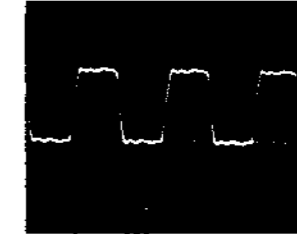
㉖ IC362 ⑤, ⑥pin 5Vp-p, 0.5μs
