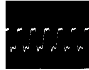
㉔ IC307 ㉓pin 6Vp-p, 0.5μs
