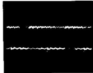
⑱ IC306 ④pin 5Vp-p, 0.2μs
