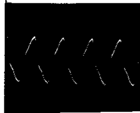
IC311 15pin 5Vp-p, 2ms
