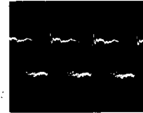
㉛ X304 ⑬pin 1Vp-p, 32.768kHz
