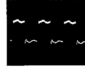
㉒ IC307 ㉒pin 5Vp-p, 1μs
