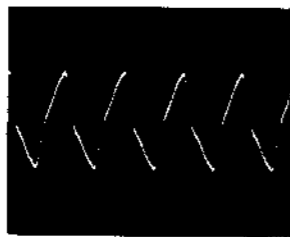
IC311 16pin 100mVp-p, 10μs
