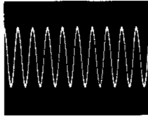
⑮ IC307 ㉑pin 5.2Vp-p, 5ms
