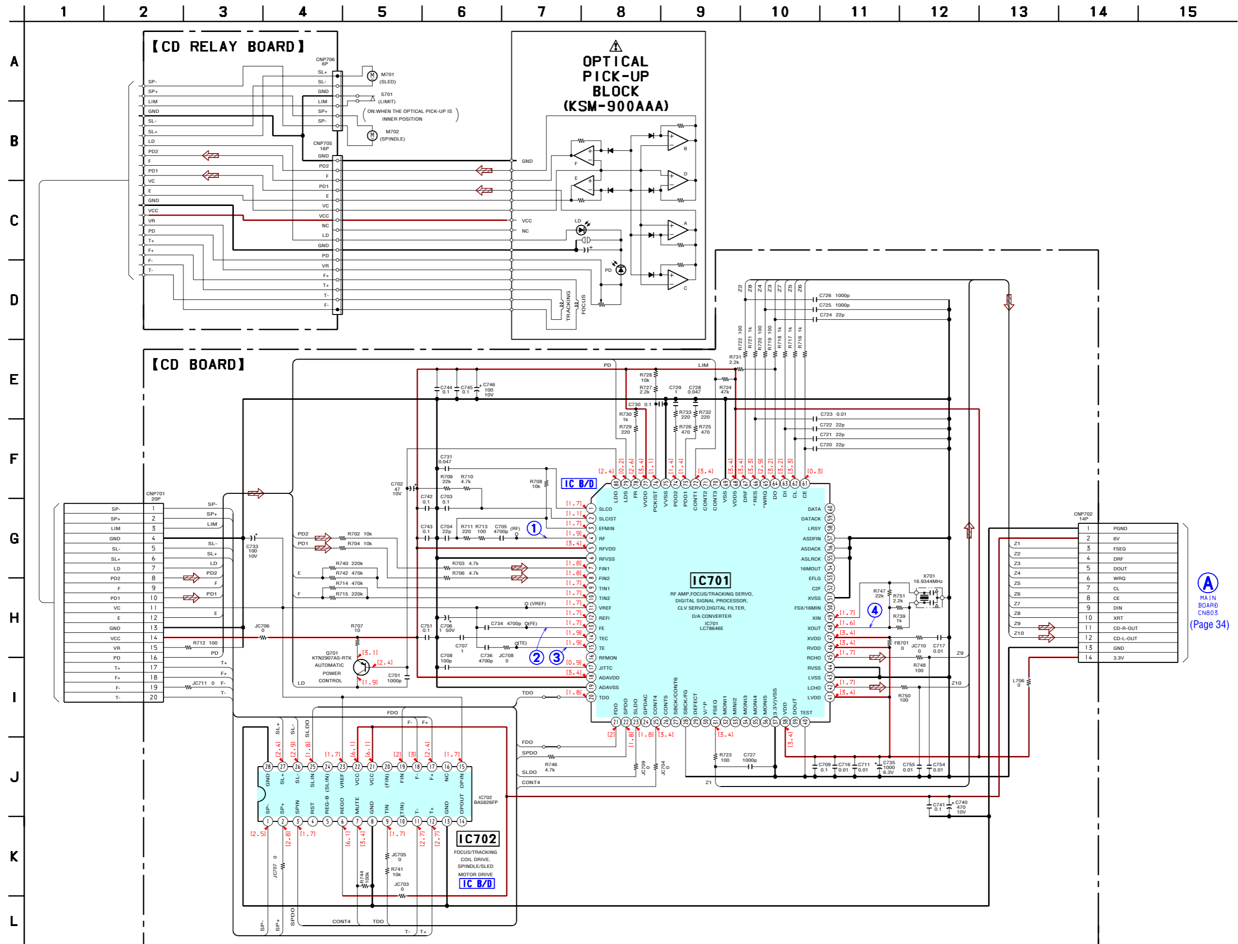
6-6. SCHEMATIC DIAGRAM – CD Section – • See page 40, 41 for IC Block Diagrams. • See page 39 for Waveforms.
