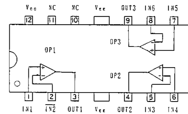
• IC4, 5 CXA1291P
