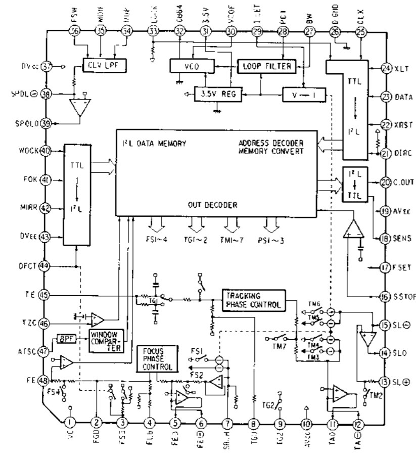
• IC3 CXA-1082BQ
