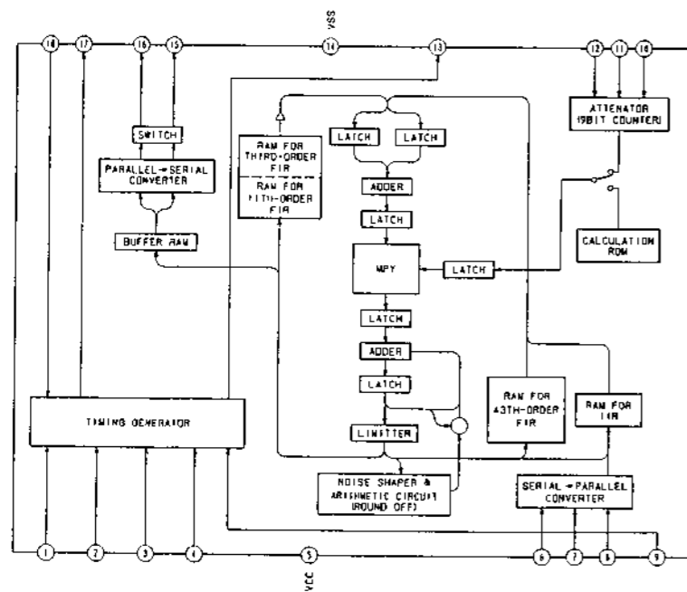
• IC9 CXD2550P
