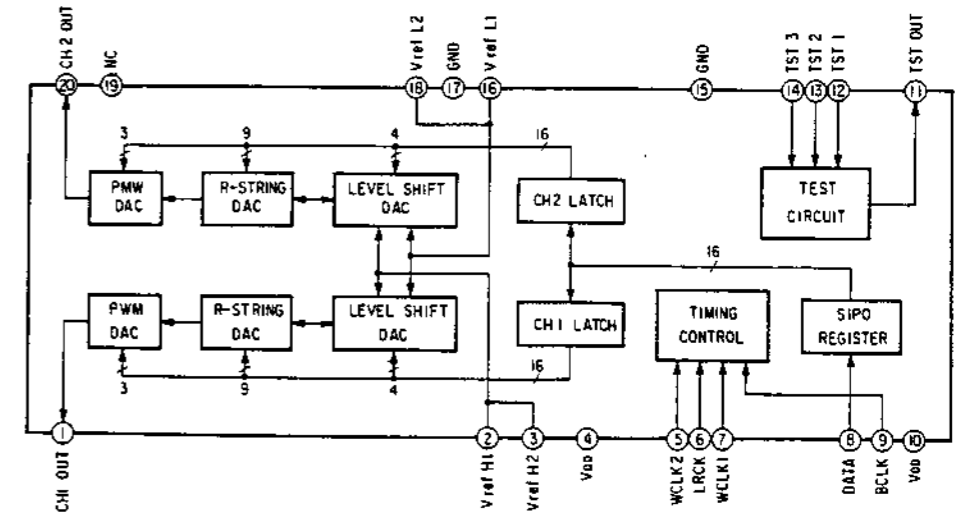
• IC10 CXD1161P-2
