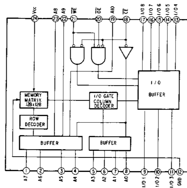
• IC1 M5294P
