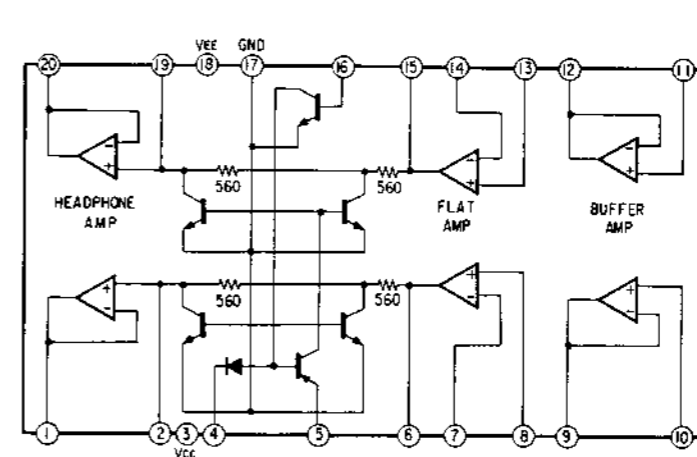
• IC11 M5204P
