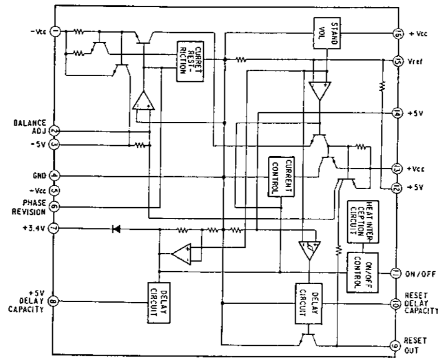
• IC1 M5294P
