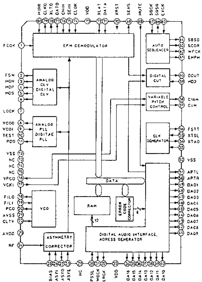
IC301 CXD2500AQ
