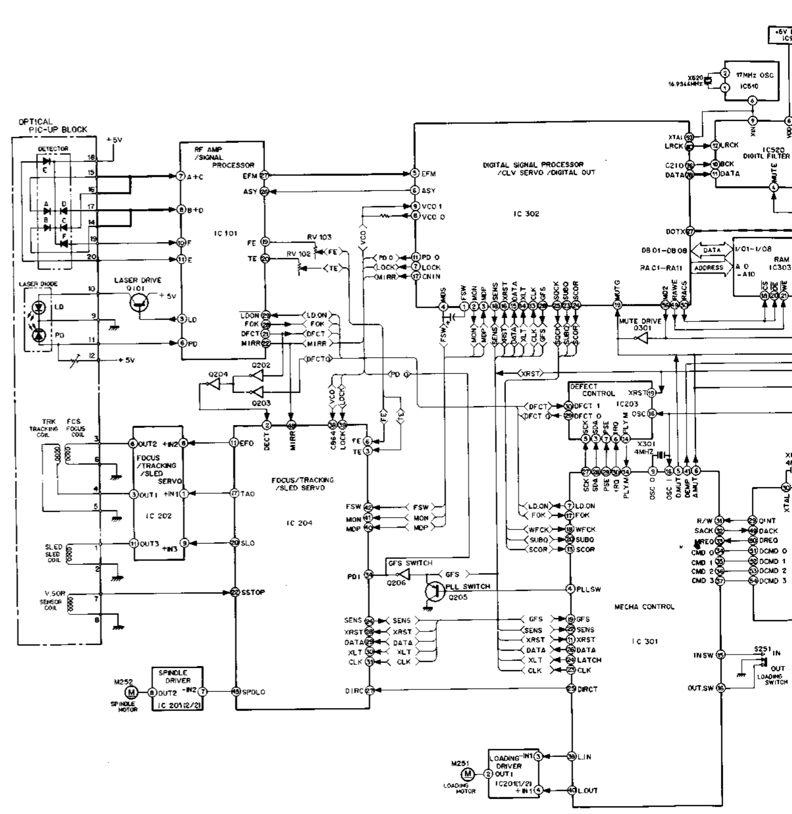
3-2. BLOCK DIAGRAM
