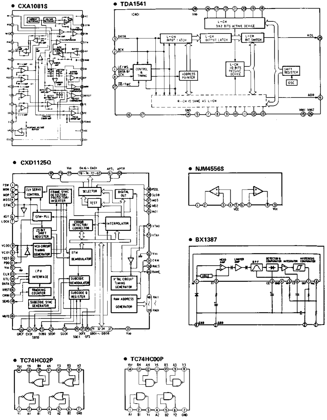
3-1. IC BLOCK DIAGRAMS
