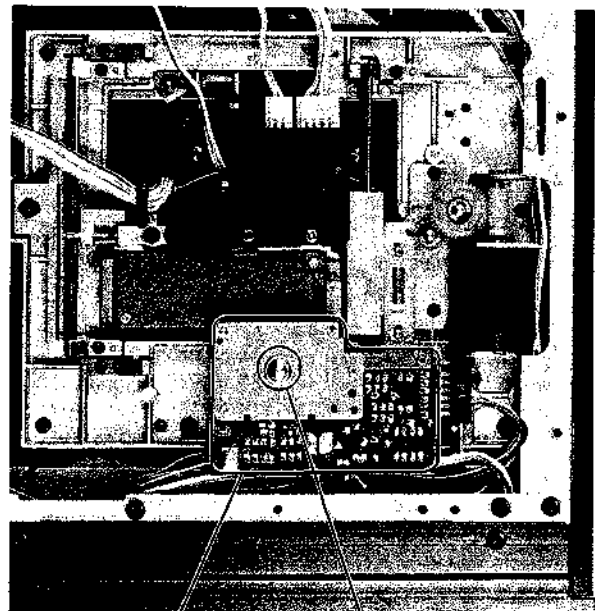
M701 disc motor motor height adjustment screw
