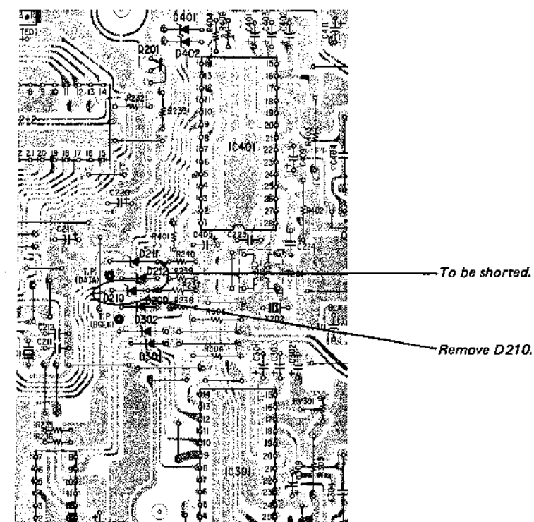
— Audio amp board (Conductor Side) —
