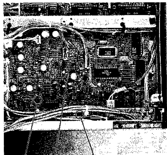
RV152 (tracking level)
