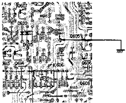
— Servo amp board — (Conductor side)
