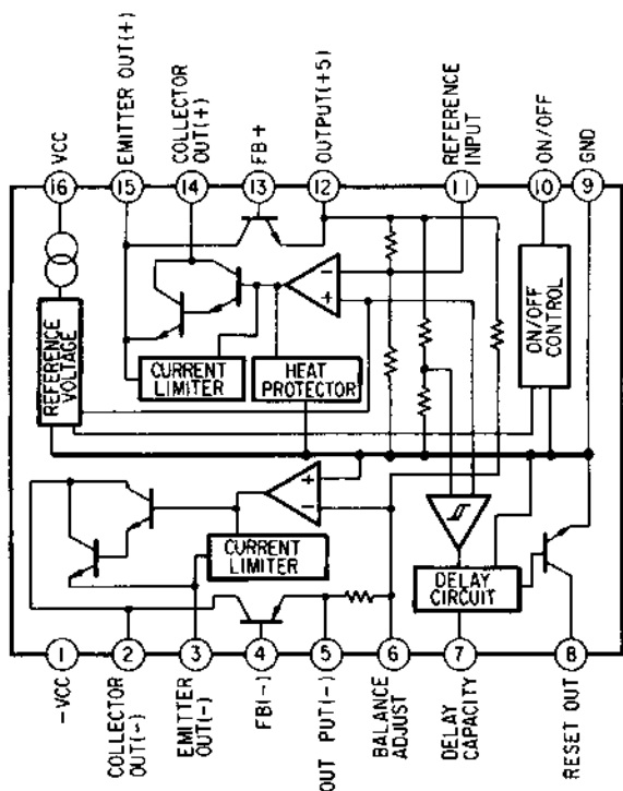
IC201 M5290P-16
