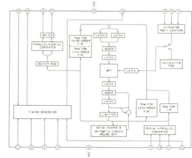
IC302 CXD2554P
