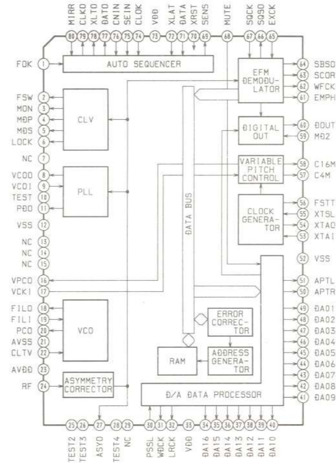
IC301 CXD2500AQ
