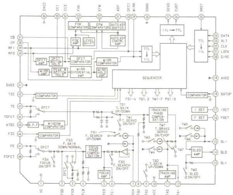
IC101 CXA1372Q
