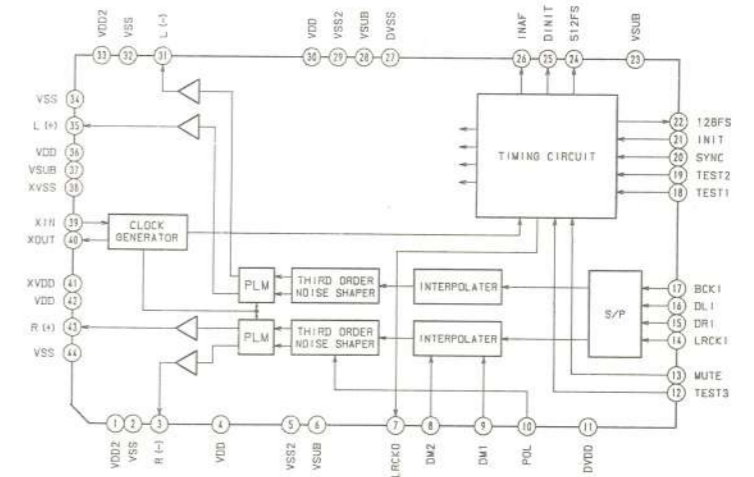
IC305 CXD2552AQ
