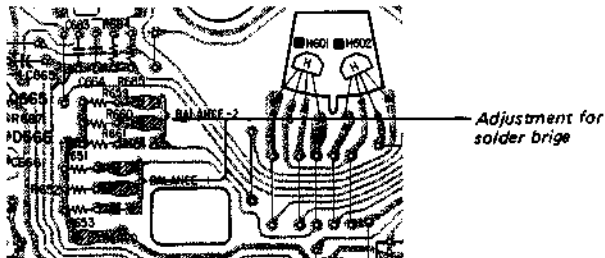
SERVO BOARD (A) (DECK side)
