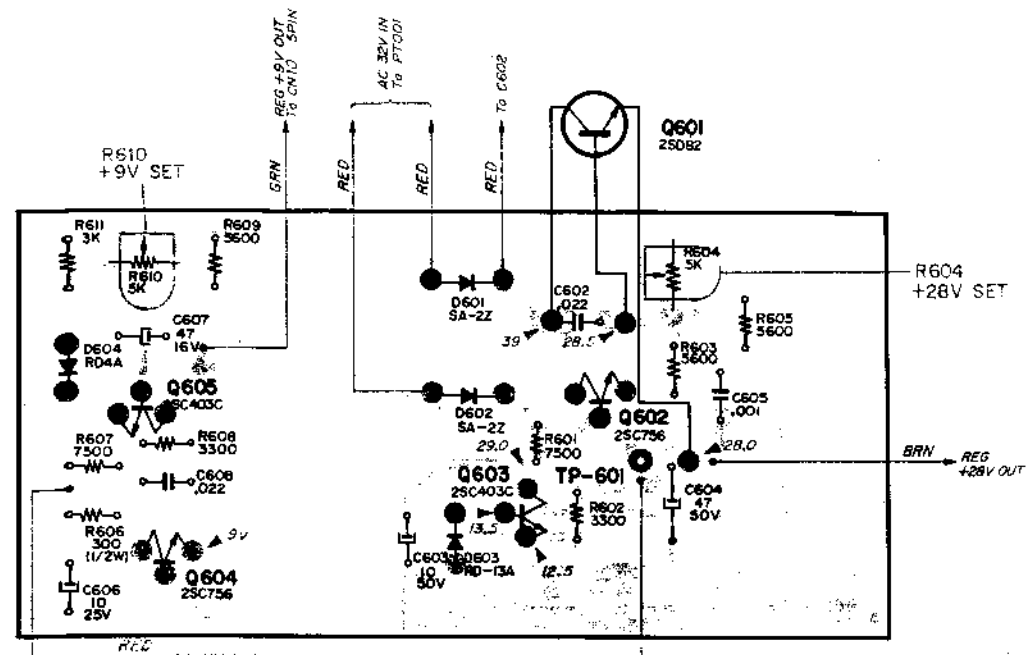
R2 VOLTAGE REGULATOR PRINTED CIRCUIT BOARD
