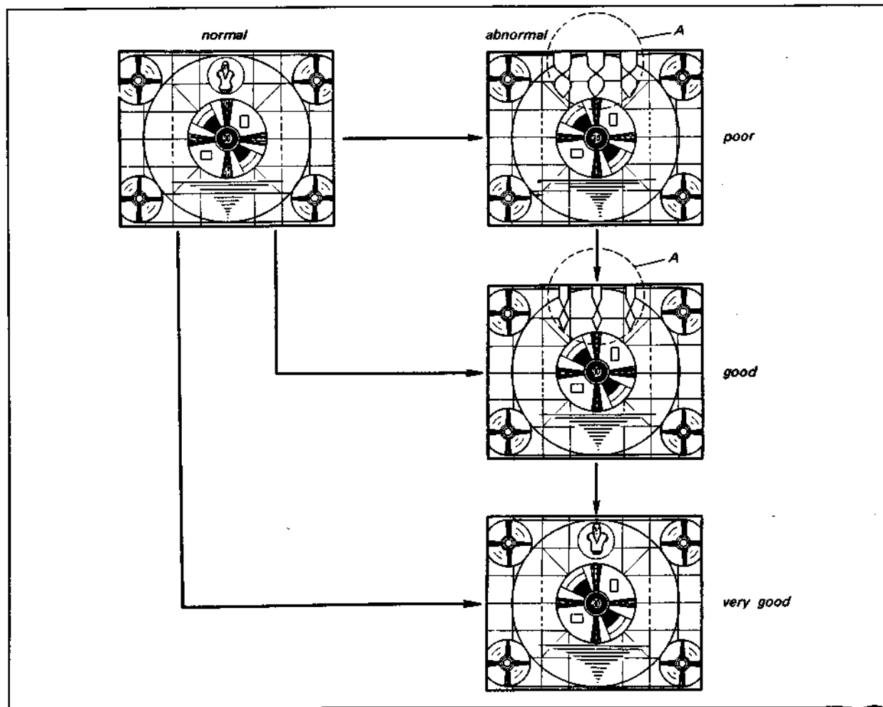
Fig. 4-7c. Picture detail for dihedral adjustment
