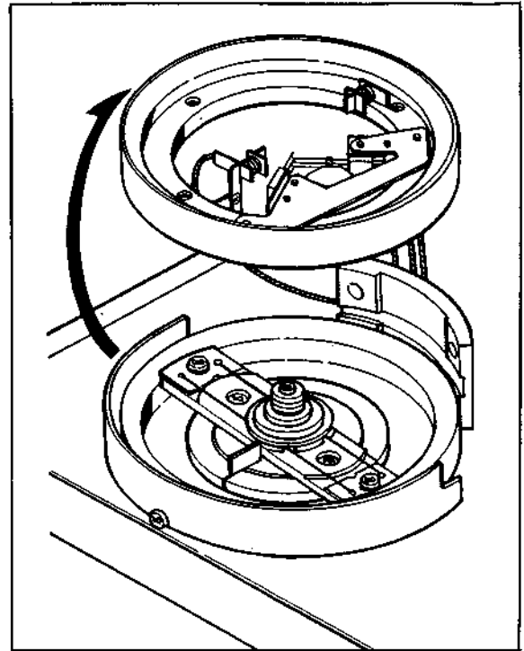
Fig. 4-5. Video head assembly removal
