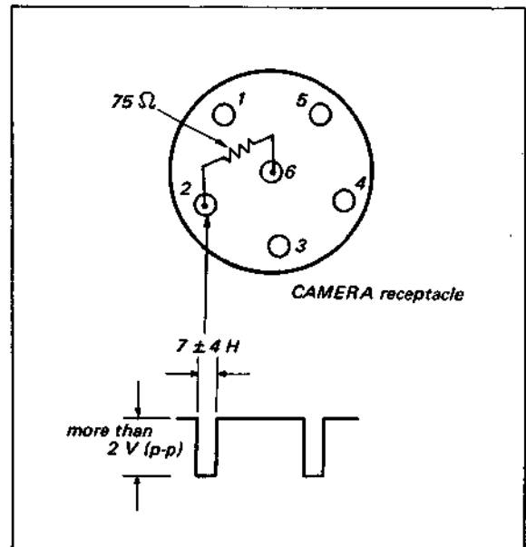
Fig. 6-13. Vertical sync for camera
