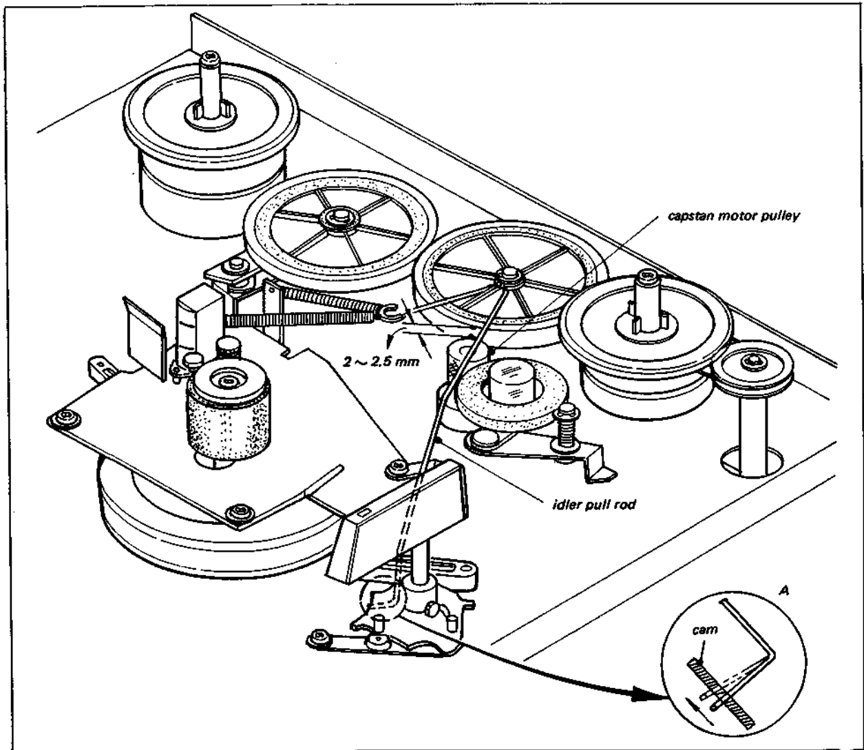
Fig. 4-17. Brake timing adjustment
