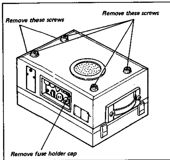
Fig. 3-1. Cabinet removal
