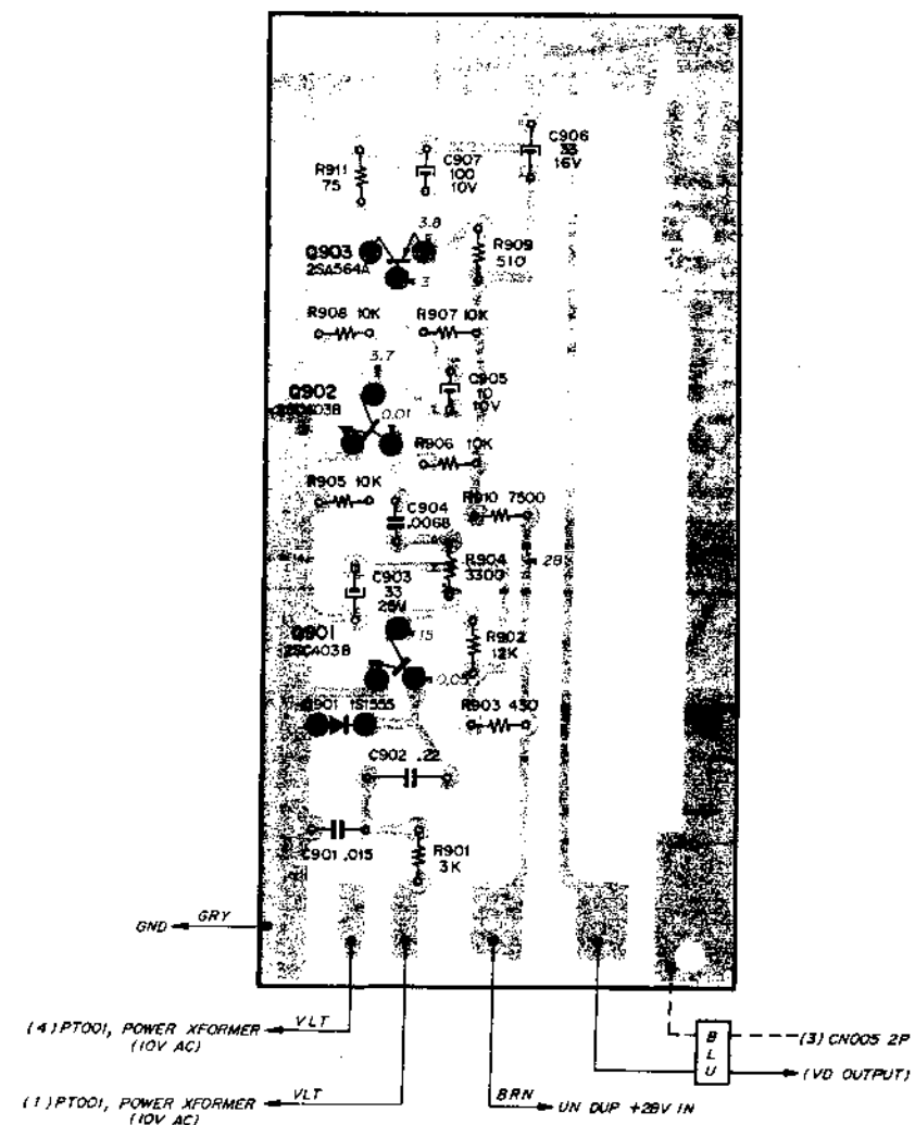
SY3 VERTICAL SYNC FORMER PRINTED CIRCUIT BOARD
