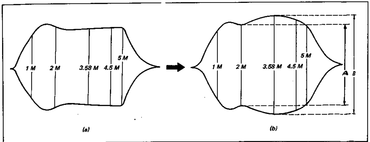
Fig. 5-5. Playback rf signal
