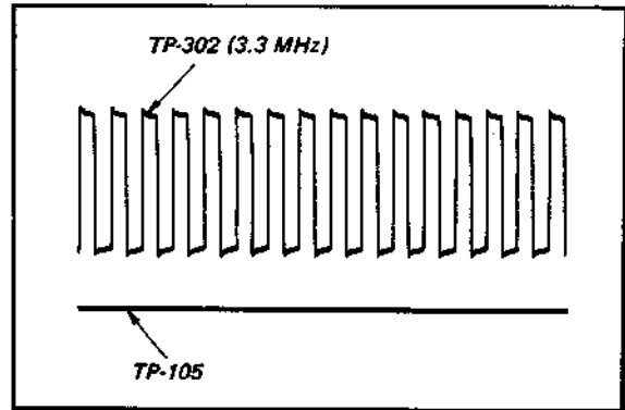
Fig. 5-2a. Waveforms in Steps 5 and 6
