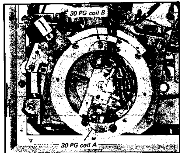
Fig. 6-8. 30 PG Coils A and B
