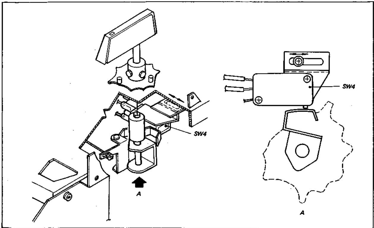
Fig. 4-25. Microswitch adjustment
