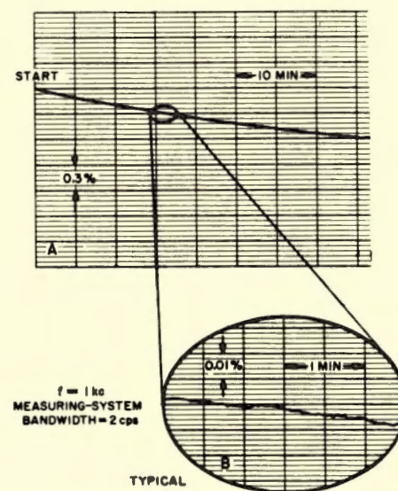
Figure C. Typical output amplitude stability of the oscillator, showing warmup drift (A) and short-term variation (B).
