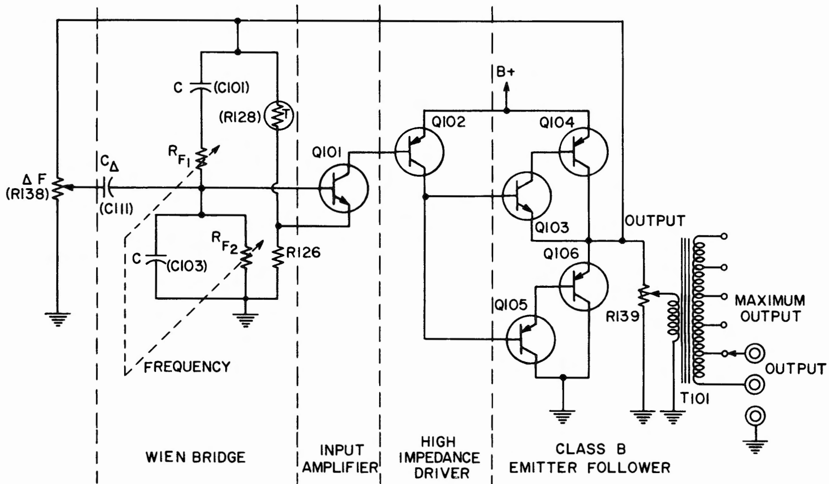
Figure 4-1. Simplified schematic diagram.
