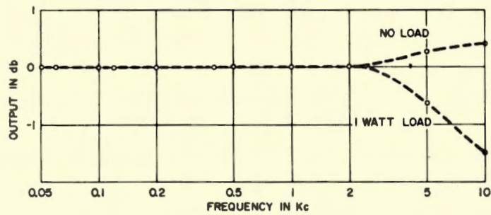
Figure A. Output of Type 1311-A as a function of frequency, loaded and unloaded (typical).
