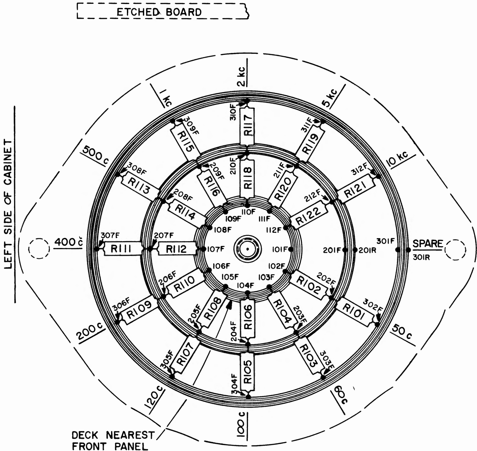
Figure 5-1. Wiring diagram for FREQUENCY switch S101.
