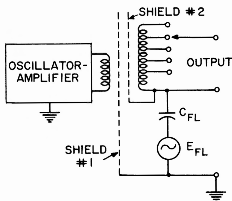
Figure 4-2. Simplified schematic diagram of output circuit.
