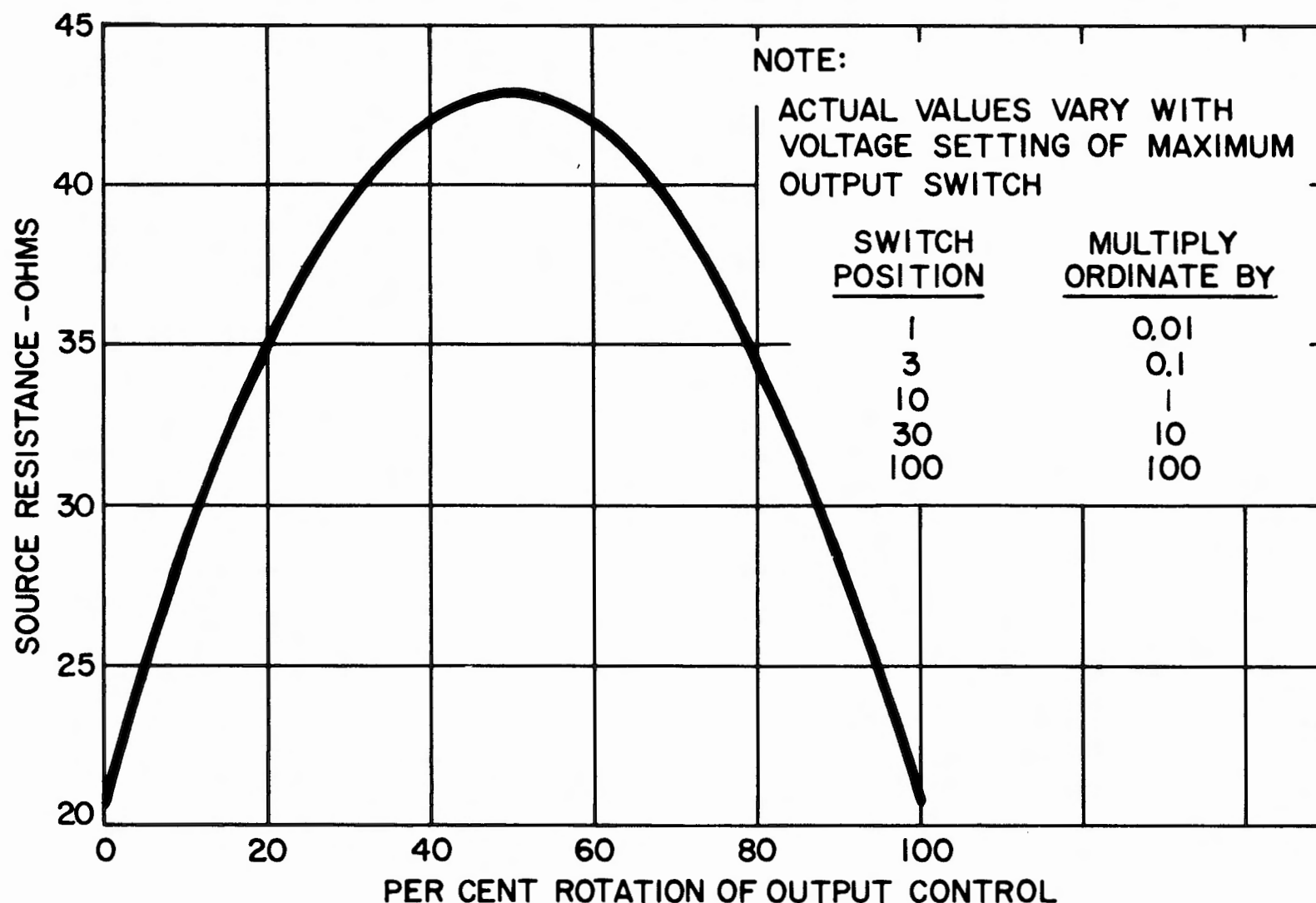
Figure 3-2. Source resistance as a function of output control settings.
