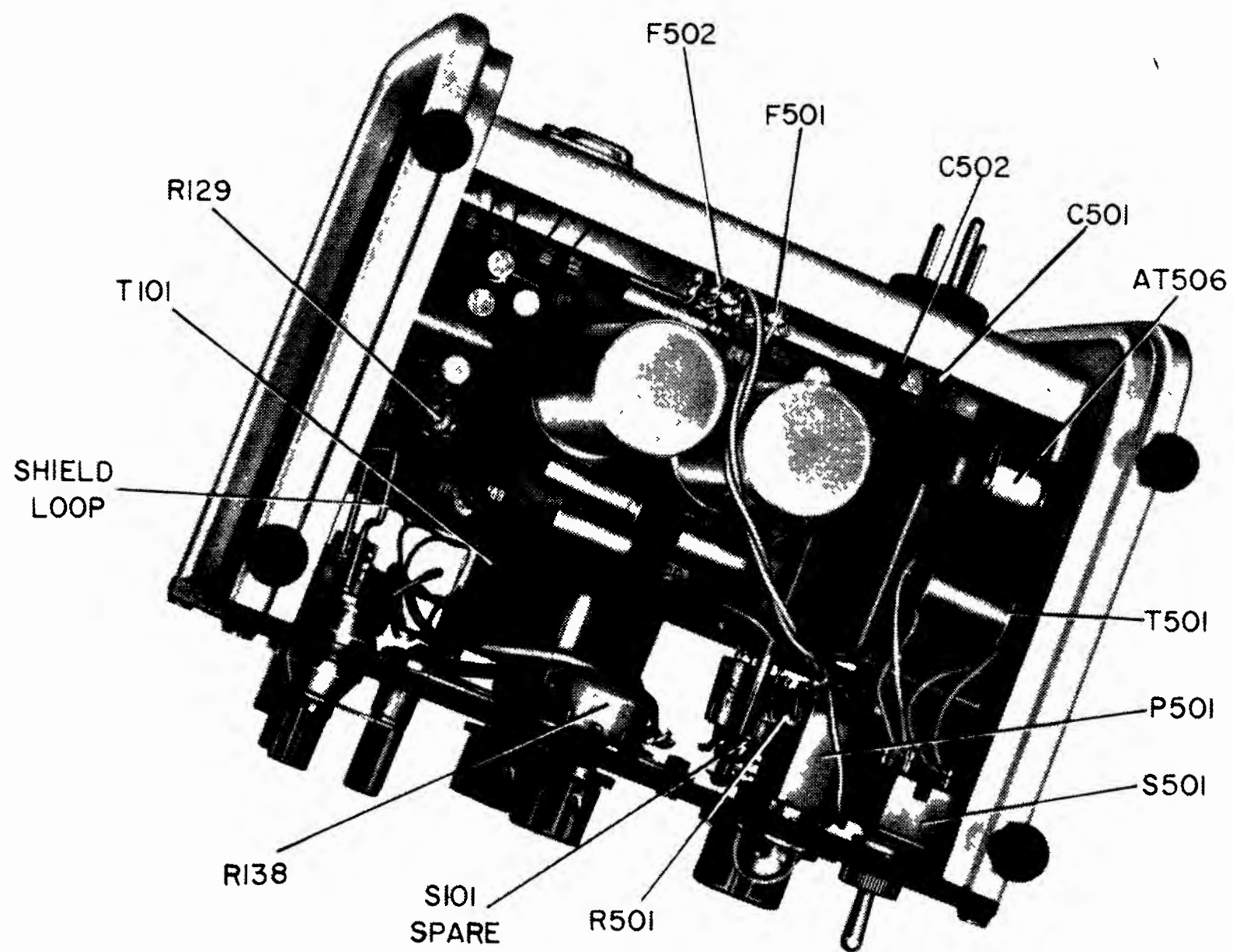
Figure 5-4. Bottom rear interior view.
