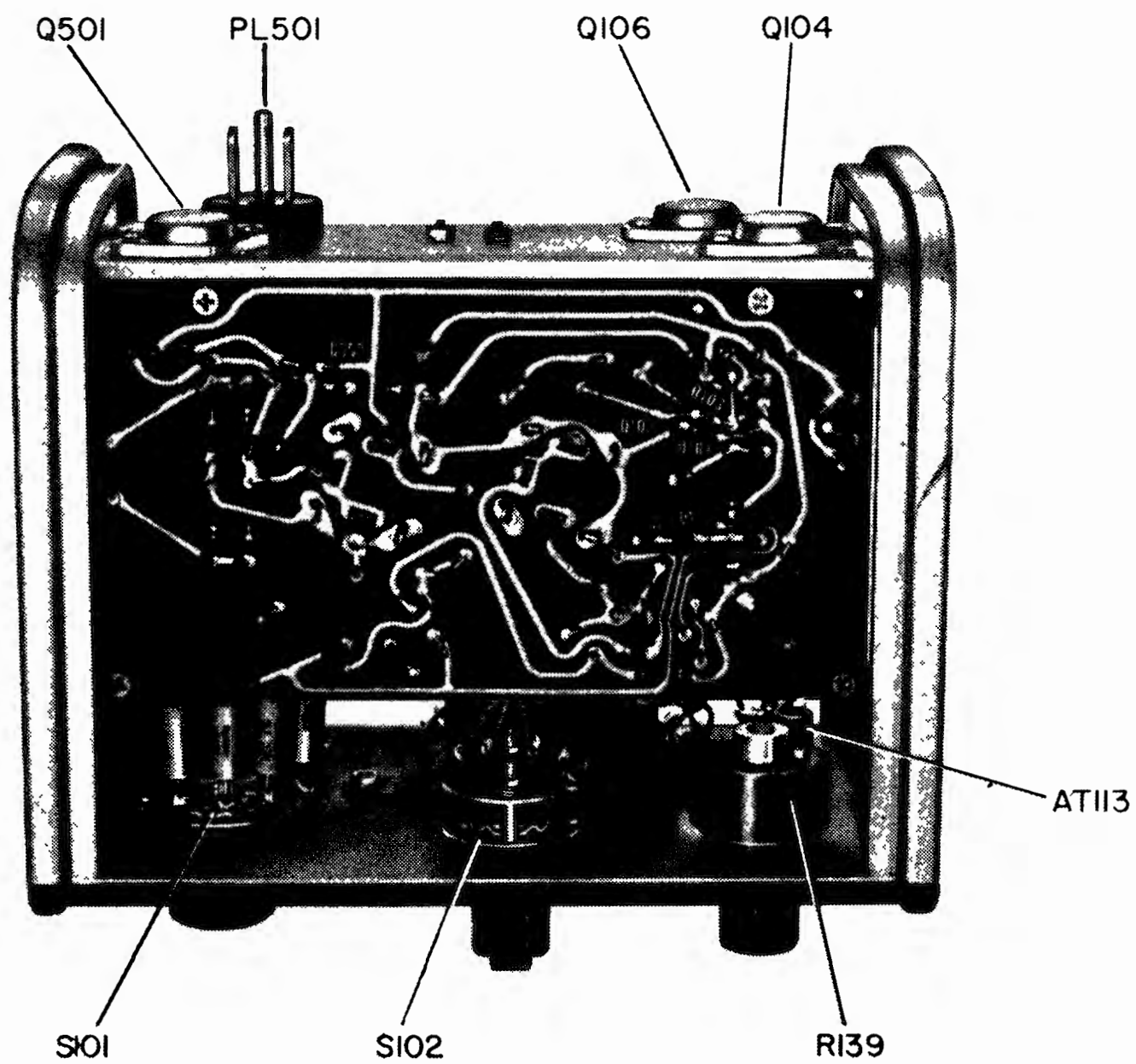
Figure 5-3. Top rear interior view.
