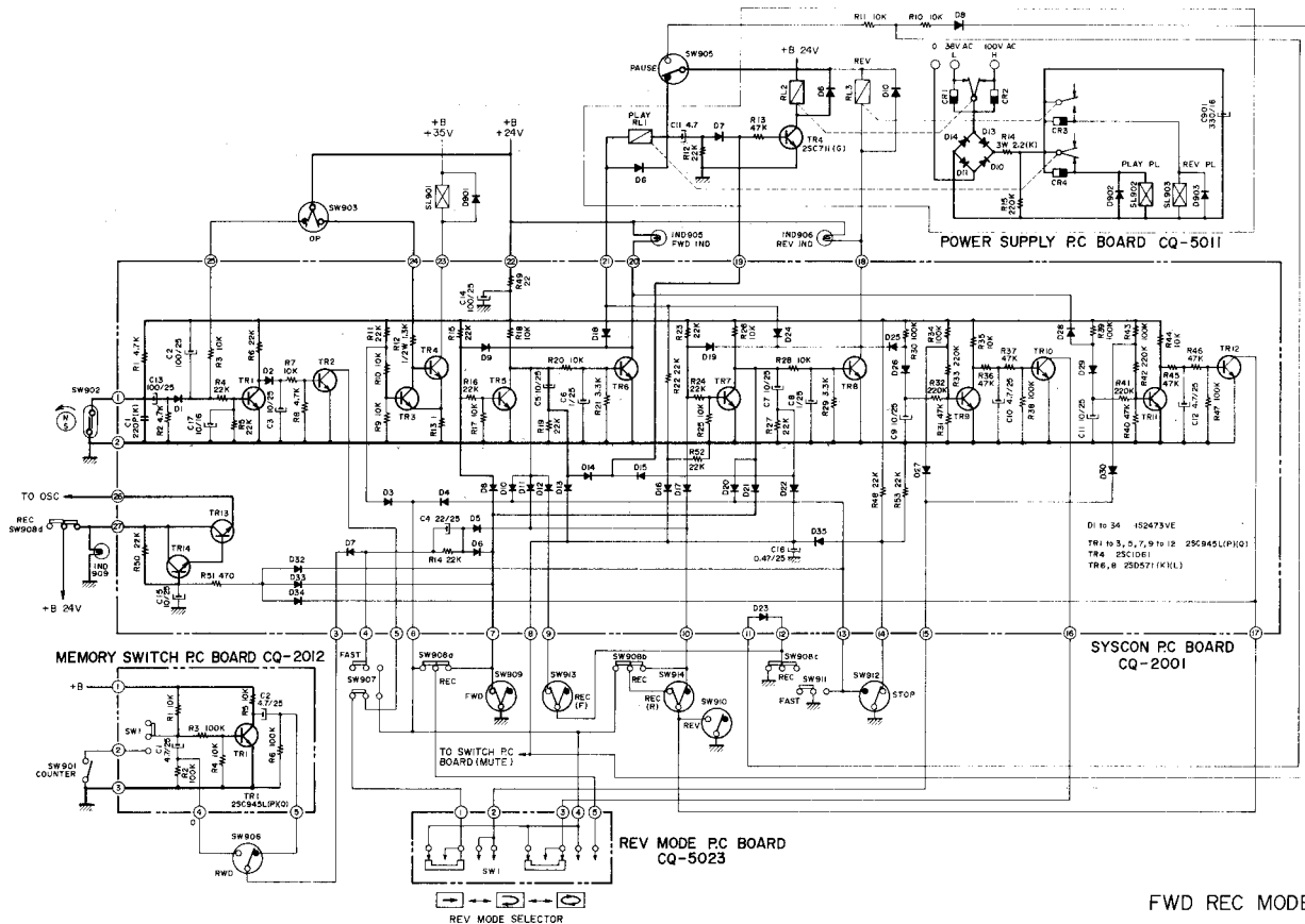
SCHEMATIC-6
