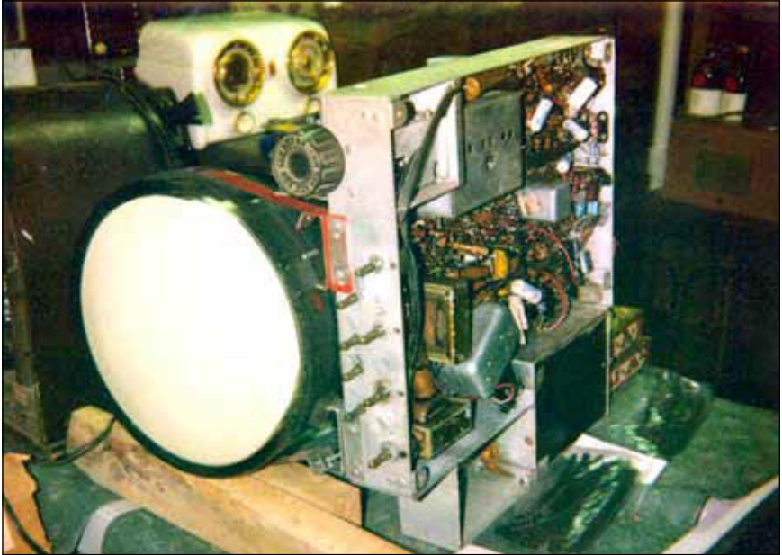
Figure 1. Raytheon 10DX24 front view.
