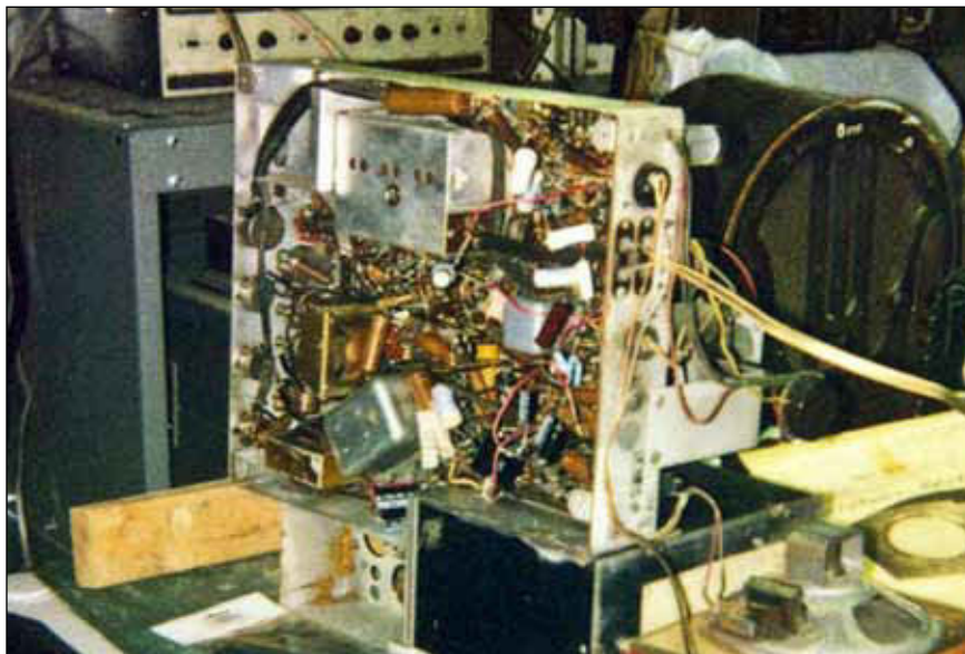
Figure 2. Raytheon 10DX24 bottom view.
