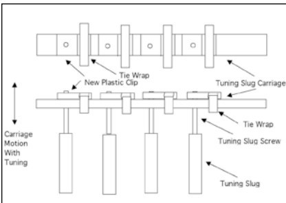
Figure 4. Slug tuned assembly with new clips.
