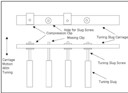
Figure 3. Slug tuned assembly.
