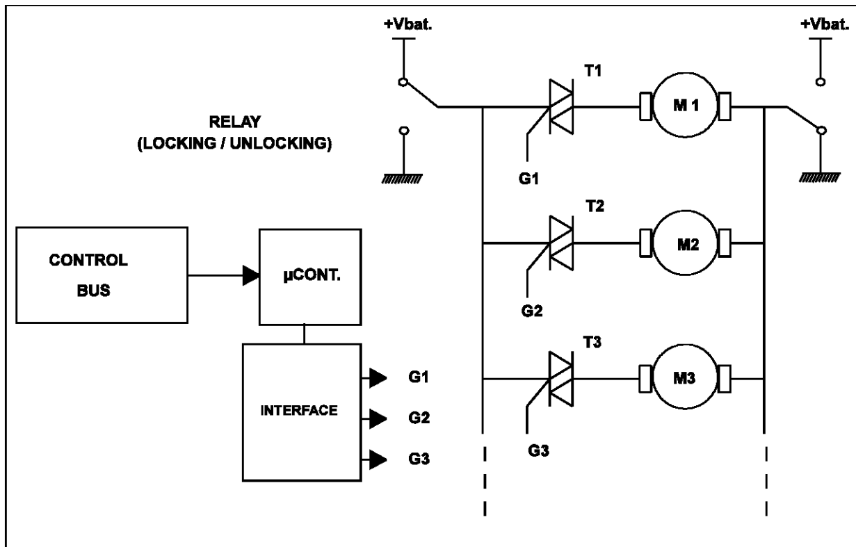
Fig. 7 : Typical circuit using triac as a bidirectionnal switch to control each door separately.
