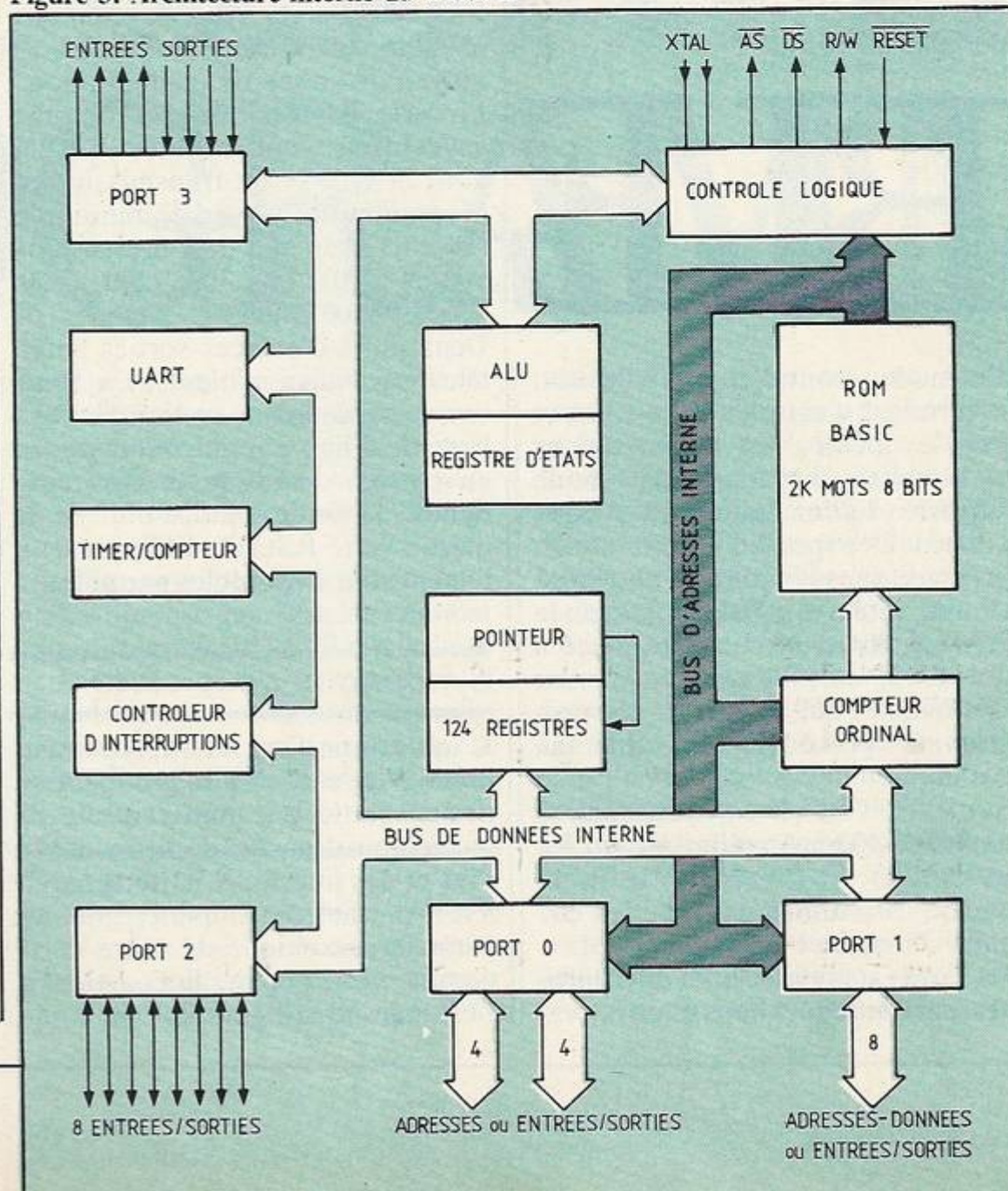
Figure 3. Architecture interne du Z 8671.
