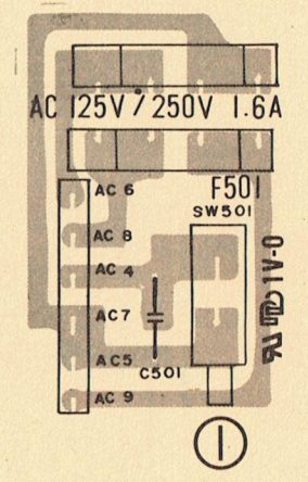
PCB switch ON/OFF Platine inter M/A LTP EIN/AUS-Schalter Platina interruptor Piastra interruttore
