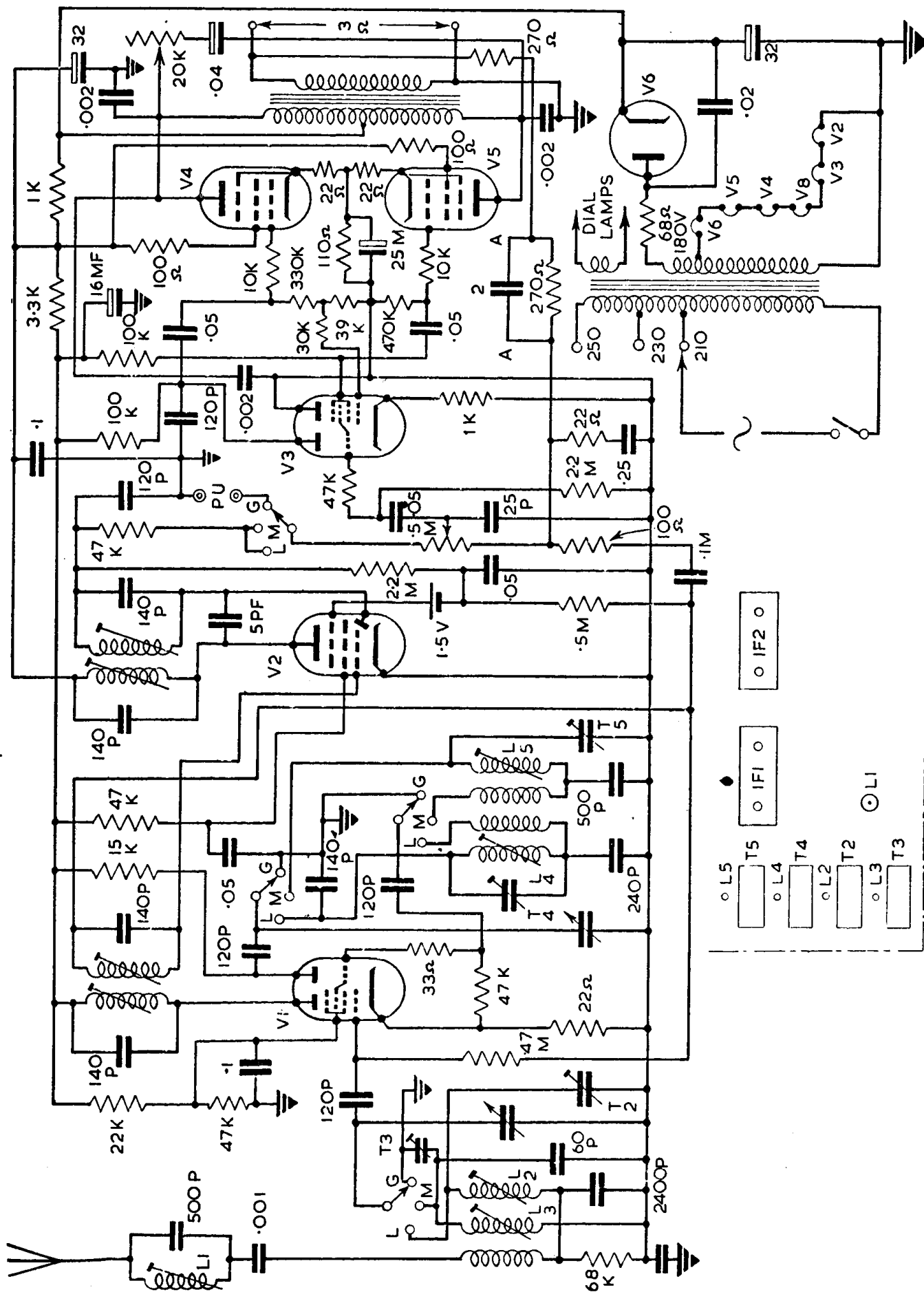
CIRCUIT DIAGRAM—AMBASSADOR MODEL 650H
