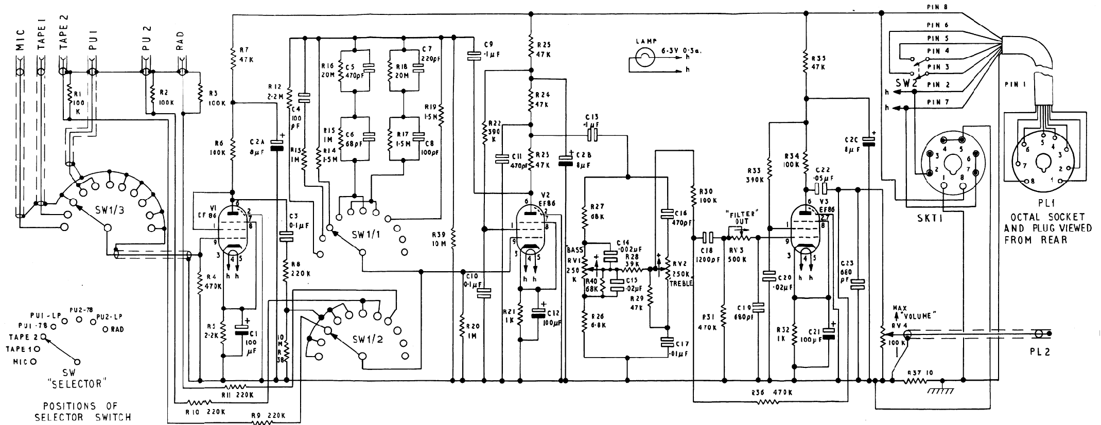
16. Circuit diagram of control unit, Type FK1PB/A1.
