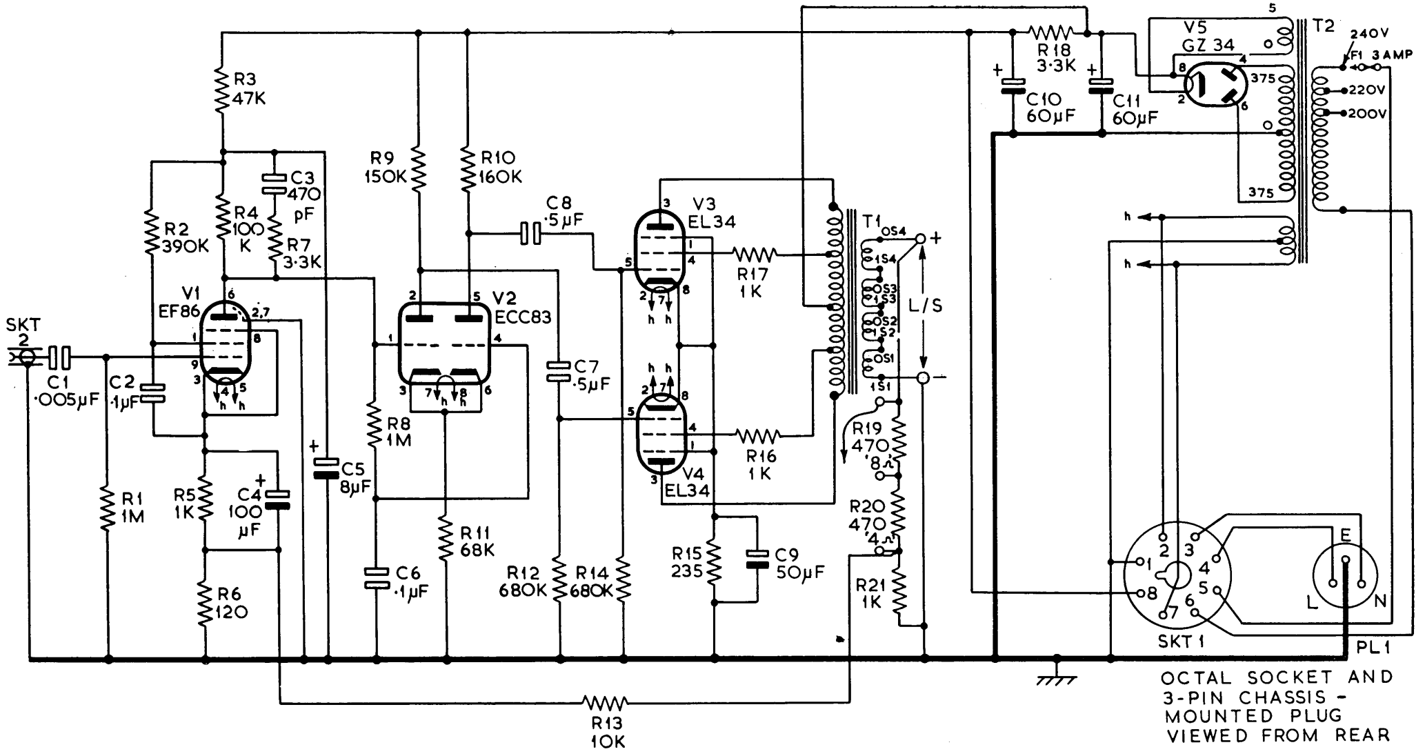
13. Circuit diagram of power amplifier, Type FK1AD/A1.
