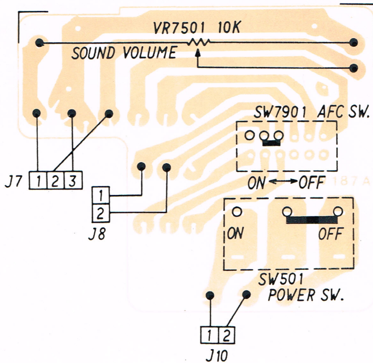
PCB5 SW187A BOTTOM VIEW
