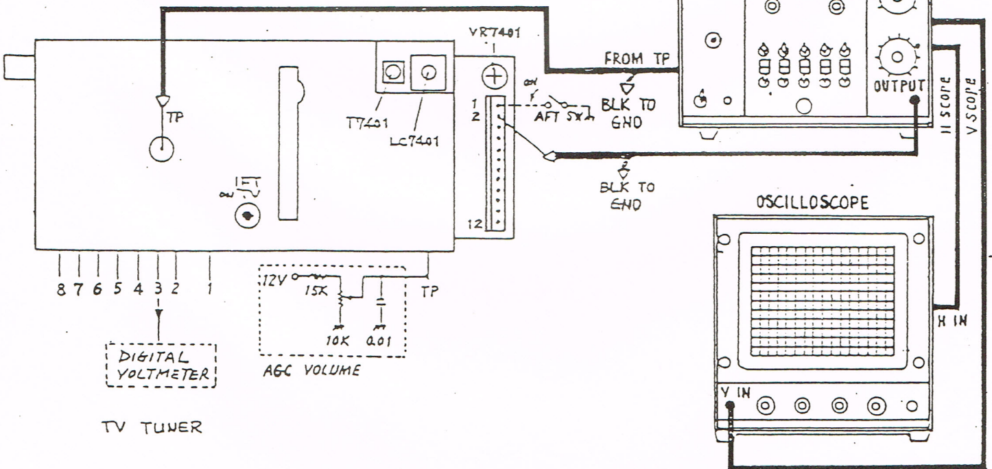
Figure 5 Video IF and AFC Alignment
