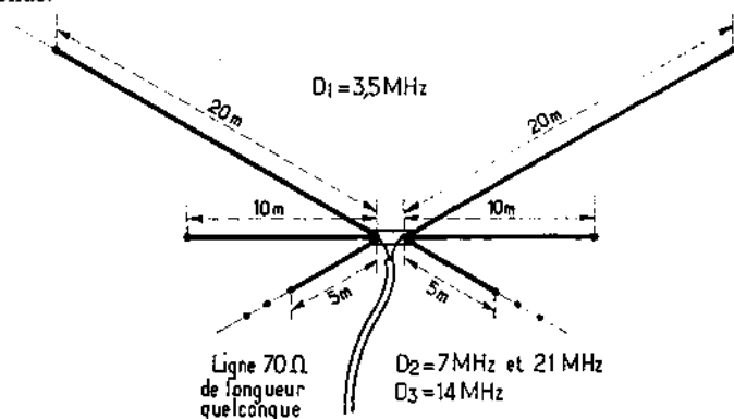
FIG. III-5 — Antenne Multi-doublet
