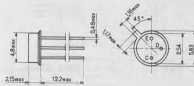
TO 48(1)
