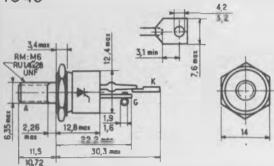
TO 49
