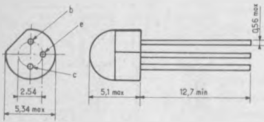
TO 127
