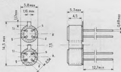
TO 94
