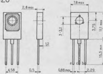
TO 202
