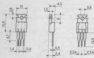
TO 220 (2)
