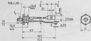
TO 106 (1)
