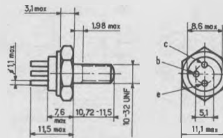
TO 60
