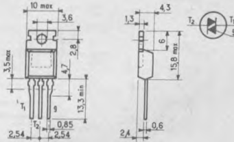
TO 220 (1)
