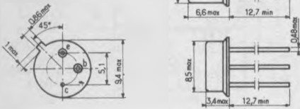
TO 41
