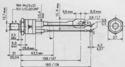
TO 94
