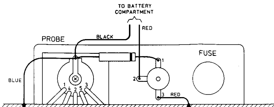
PM 2517E/01 Serial numbers DM900 and following
