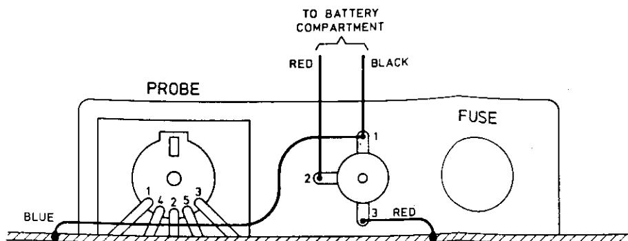
PM 2517E/01 Serial numbers DM600 – DM900
