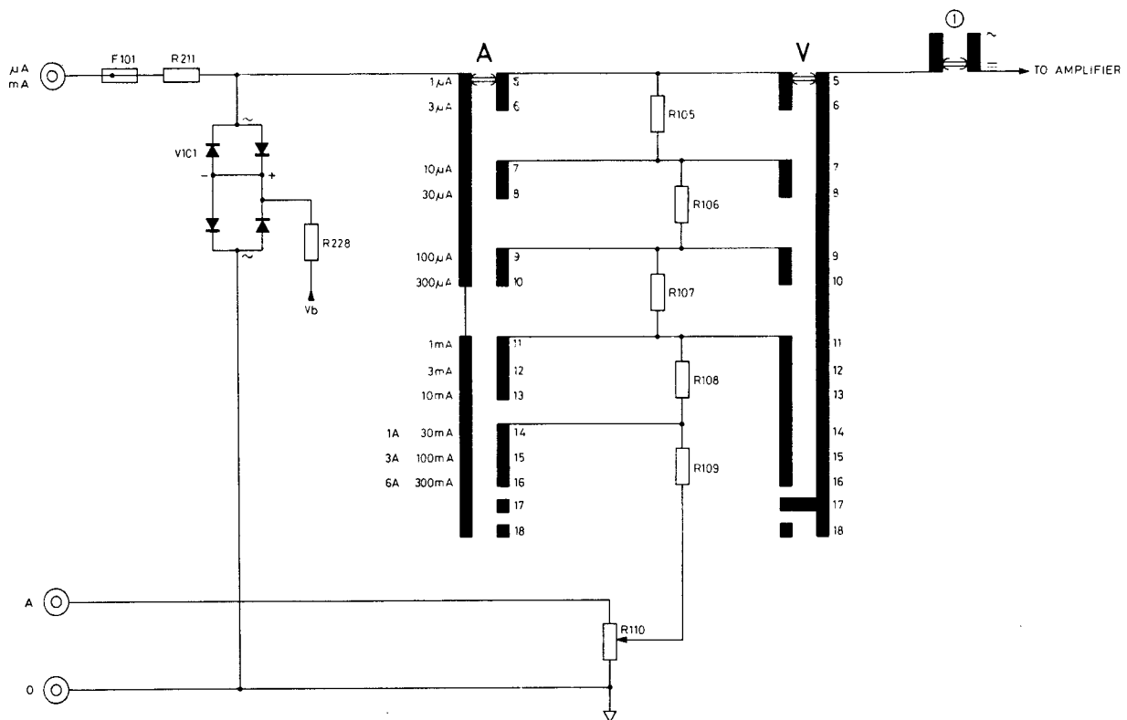
Fig. 10. A \equiv , and A \sim shunts
