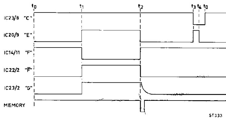
Fig. 17. Sequence diagram memory signal
