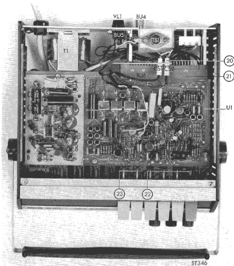
Fig. 34. Top view (cabinet removed)
