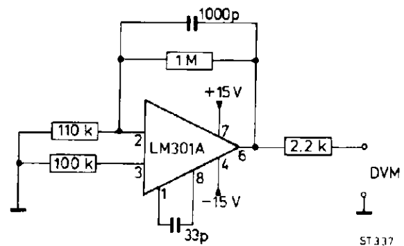
Fig. 26. Circuit for selection of IC4
