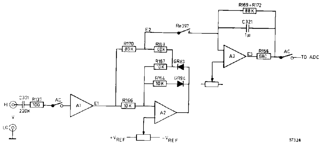
Fig. 7. Alternating voltage measuring circuit
