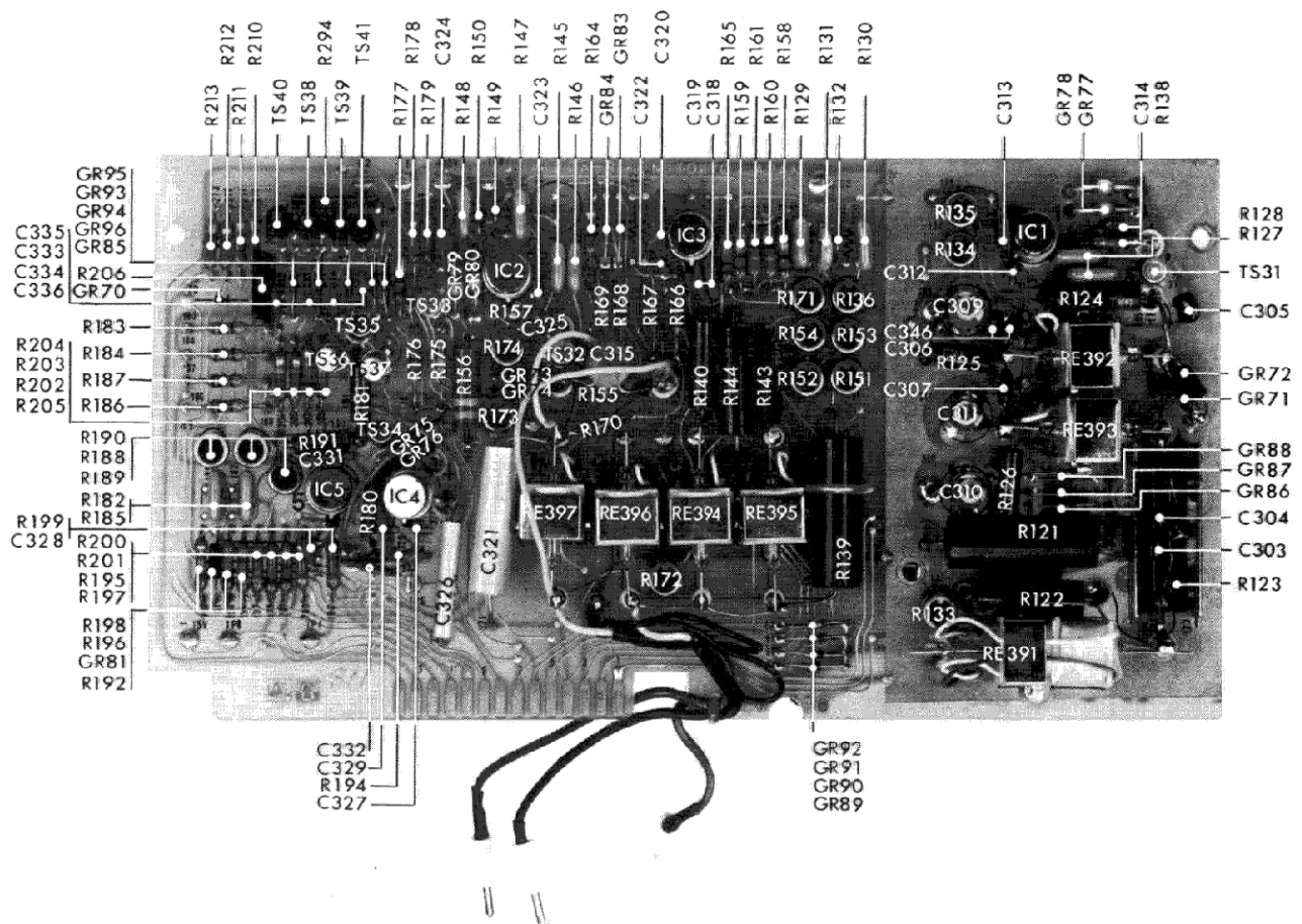
Fig. 37. Printed wiring board U1
