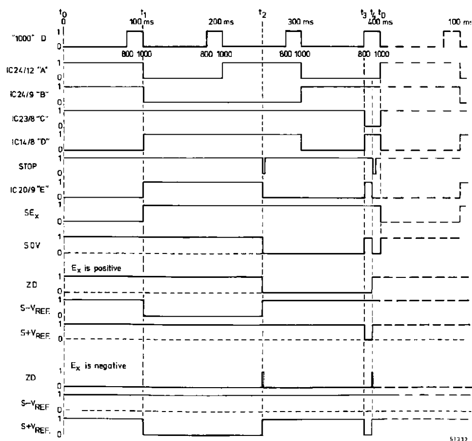
Fig. 14. Sequence diagram
