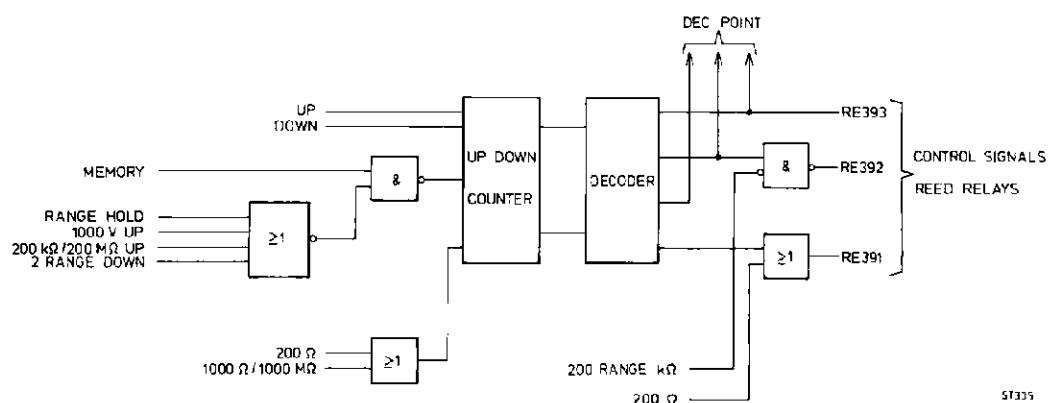
Fig. 22. Block diagram autorange circuit
