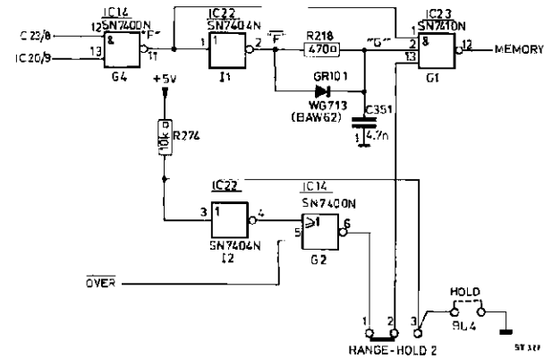
Fig. 16. Memory signal generator
