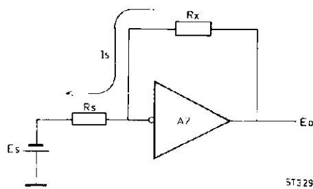
Fig. 8. Principle of resistance measurements
