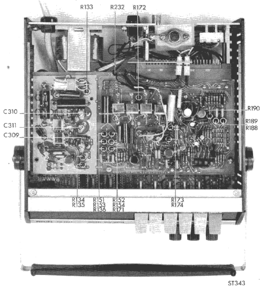
Fig. 30. Indications of adjusting elements
