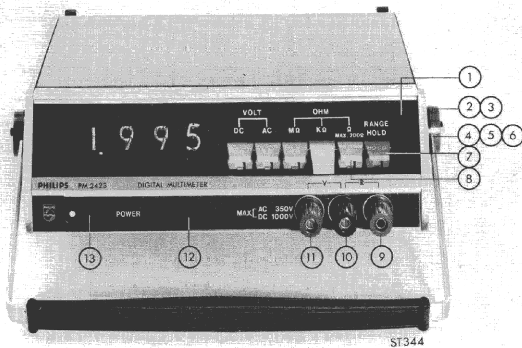
Fig. 32. Front view with item numbers
