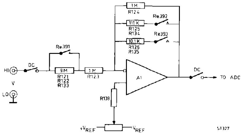
Fig. 6. Direct voltage measuring circuit
