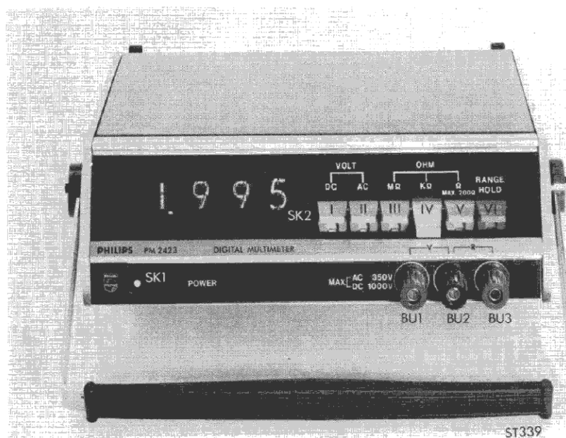
Fig. 4. Front view
