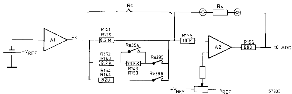
Fig. 9. Resistance measuring circuit
