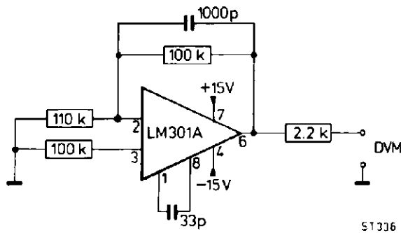
Fig. 25. Circuit for selection of IC1, IC2 and IC3
