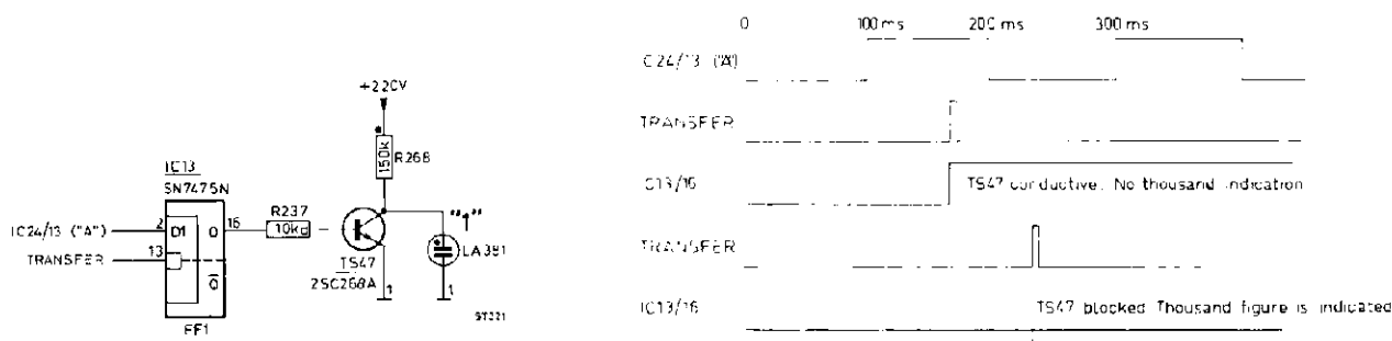
Fig. 21. Thousands indication
