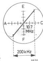
Fig. 24. Discriminator curve
